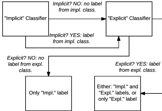
Figure 1: Classification system using two classifiers and negative examples (the order of the two classifiers does not matter as they are independent).
