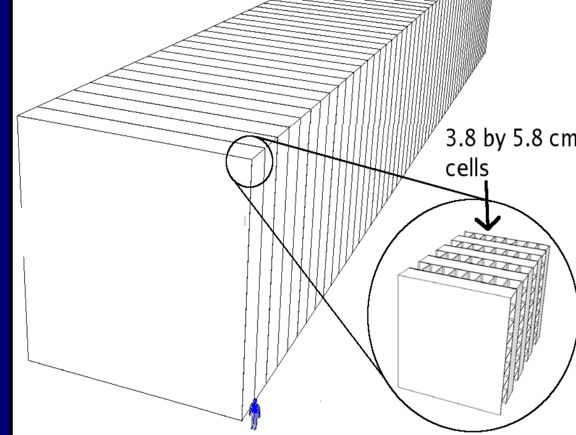
Figure 1. Diagram of far detector. Adjacent planes of modules are oriented perpendicularly to give x, y resolution, as depicted in diagram inset.
