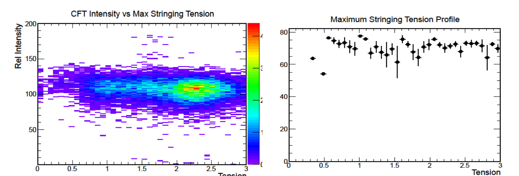
Figure 5. Two dimensional histogram and profile of relative transmitted light and maximum stringing tension as obtained by the CFT are shown. The profile shows the mean of each x (x=bin size) bin with error bars indicating a 1 sigma deviation from the mean.
