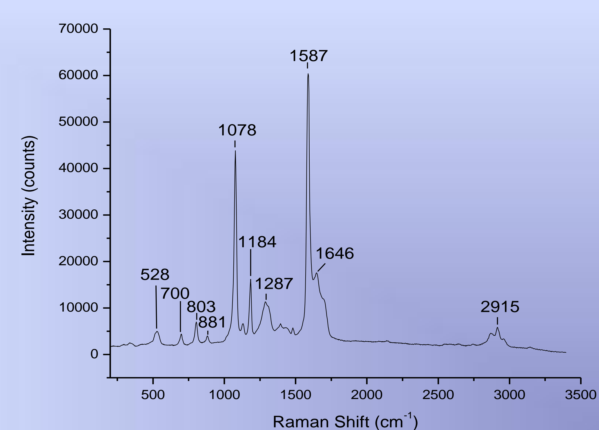
Figure 2. SERS spectrum of 4-MCBA on Ag colloid solution
