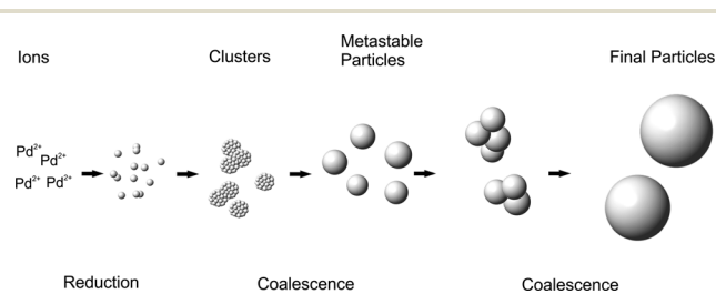
Fig. 3 Schematic illustration of the deduced growth mechanism of Pd-NPs.
