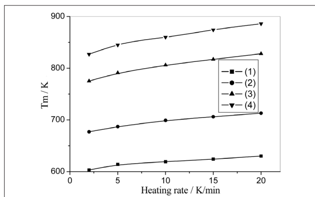
Figure 5. Dependence of T_m on heating rate for the processes (5) – (8) occurring during the chalcopyrite concentrate oxidation
