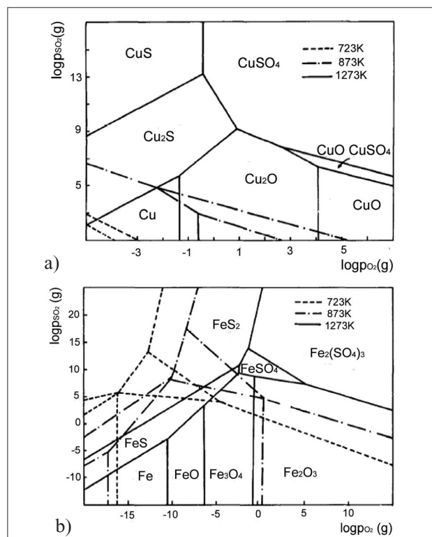
Figure 4. The Kellogg diagrams for Cu-S-O (a) and Fe-S-O (b) systems at the temperatures typical for oxidation roasting process - 723, 873 and 1273 K [15]
