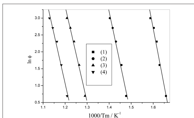
Figure 7. Linear correlation between \ln \phi and 1/T_m for the processes (5) – (8) occurring during the chalcopyrite concentrate oxidation
