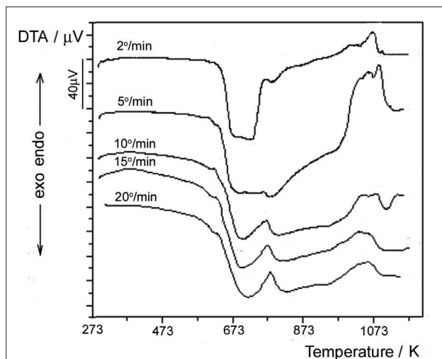
Figure 1. DTA curves of chalcopyrite concentrate oxidation at different heating rates
