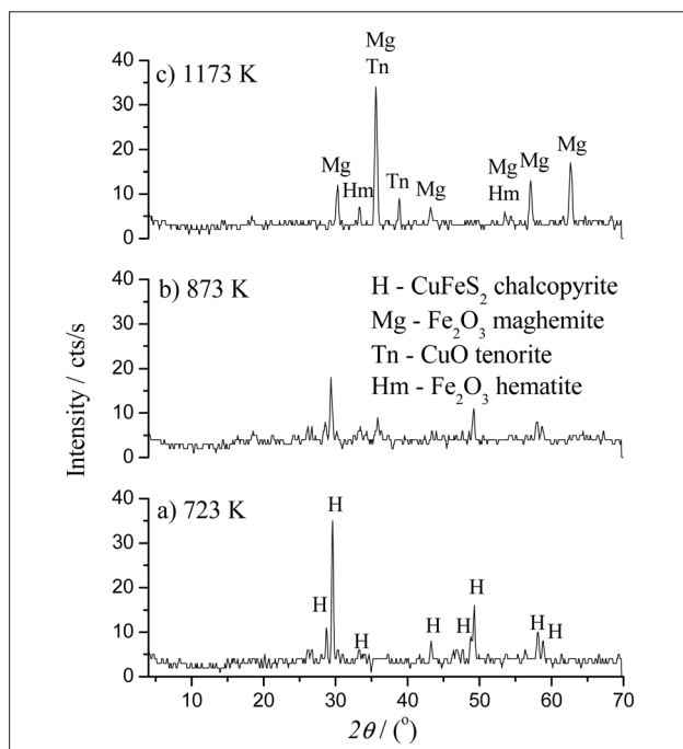
Figure 3. X-ray recordings of the chalcopyrite concentrate oxidation products at 723 K (a), 873 K (b) and 1173 K (c)
