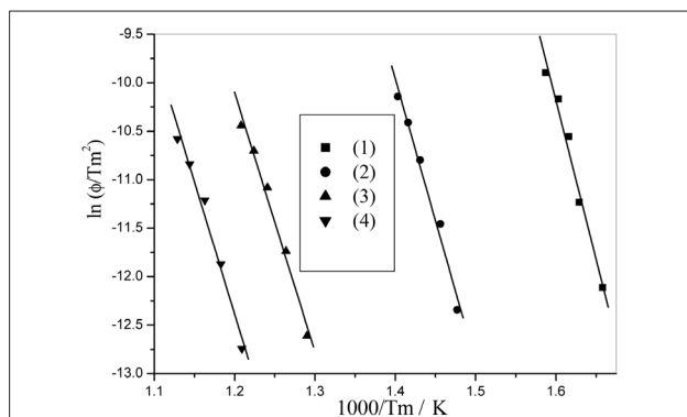
Figure 6. Linear correlation between \ln(\phi/T_m^2) and 1/T_m for the processes (5) – (8) occurring during the chalcopyrite concentrate oxidation
