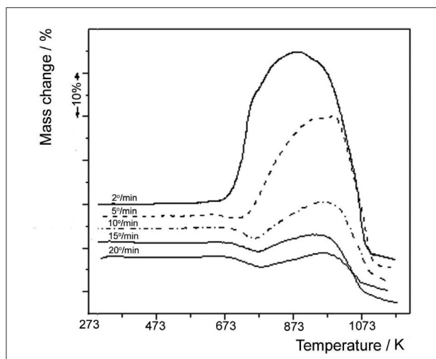
Figure 2. TG curves of chalcopyrite concentrate oxidation at different heating rates
