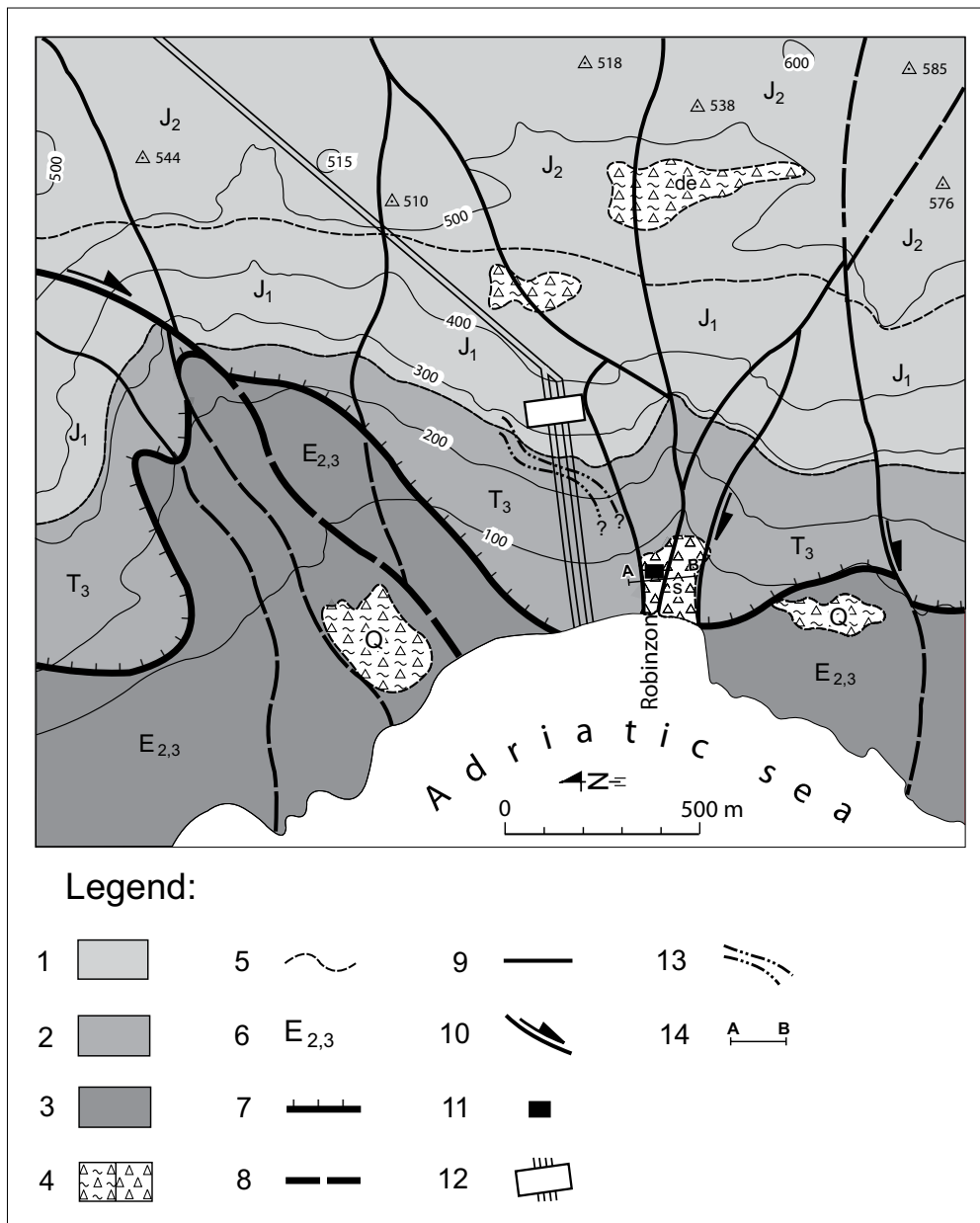
Fig. 2 Simplified hydro-geological map of the study area. Legend: 1 – permeable carbonate rocks; 2 – poorly permeable carbonate rocks; 3 – impermeable clastic rocks; 4 – permeable clastic rocks; 5 – geological boundary; 6 – chronostratigraphic unit; 7 – thrust fault; 8 – the Slivnički fault; 9 – normal fault; 10 – tear faults; 11 – the Robinzon Spring; 12 – the Dubrovnik power plant; 13 – caves; 14 – hydrogeological cross-section.
