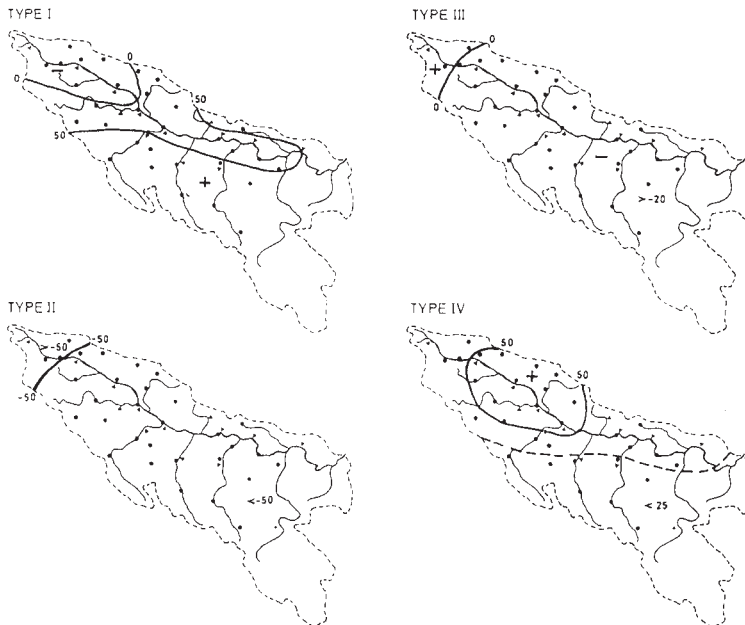
Figure 4. Anomaly patterns of monthly precipitation over the Sava river basin
