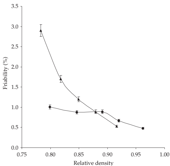
Fig. 4. Friability vs. relative density for paracetamol tablets containing 3.0% ( m/m ) binder: ▲ Albizia gum, ● gelatin (mean ± SD, n = 3).
