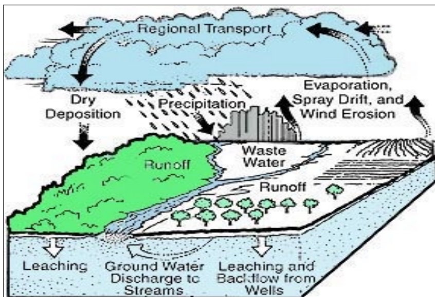
Figure 1: Pathways of pesticide movement in the hydrologic cycle [2]
