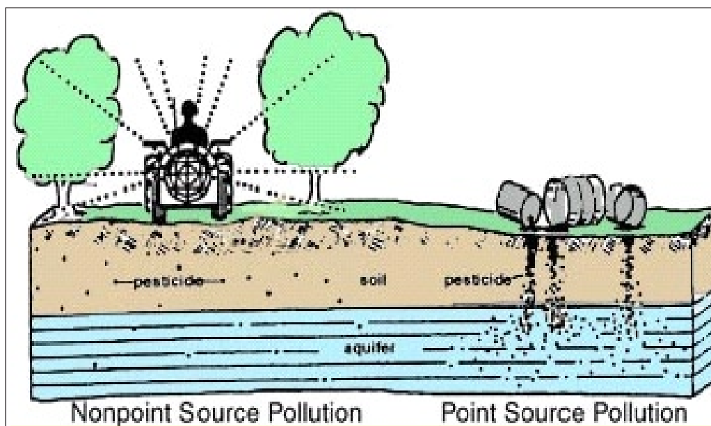
Figure 2: Pesticides can enter water supplies from point sources or from nonpoint sources [2]
