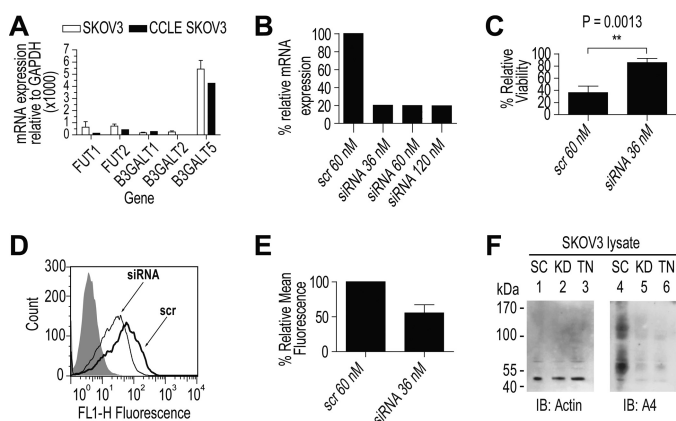
Figure 11. Effects of siRNA knockdown of B3GALT5 in SKOV3. Data were taken 72 h after siRNA was reverse-transfected into SKOV3. A , comparison of expression levels of genes responsible for H type 1 found in this study by qRT-PCR ( open columns ) versus data from the CCLE ( filled columns ) for SKOV3. Error bars show 1 S.D. from three biological replicates. B , effect of increasing concentration of siRNA versus scramble on mRNA of B3GALT5 measured by qRT-PCR and effect on cell yield as measured by hemocytometer. C , effect of siRNA knockdown on mAb-A4 cytotoxicity. Data were from three biological replicates (**, p = 0.0013 ). D , binding profile of mAb-A4 to SKOV3 transfected with 36 nM B3GALT5 siRNA or scramble ( scr ). E , change in relative mean fluorescence of mAb-A4 to SKOV3 transfected with 36 nM B3GALT5 siRNA or scramble ( scr ). Data were from three biological replicates. F , effect of 36 nM siRNA knockdown ( KD ) or 5 \mu\text{g}/\text{ml} tunicamycin ( TN ) on anti- \beta -actin and mAb-A4 Western blot of SKOV3 whole cell lysate, compared with scramble ( SC ). The samples were equally split for staining with anti- \beta -actin (42 kDa) and mAb-A4. Molecular mass markers in kDa are shown on the left. IB , immunoblot.
