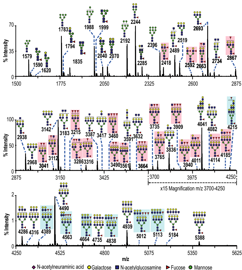
Figure 5. Types of potential mAb-A4 epitopes in the N -glycome of SKOV3. Partial mass spectrum of permethylated desialylated N -glycans from 10 million SKOV3 cells, acquired by MALDI-TOF in positive mode (50% acetonitrile fraction). Intensity was normalized to the m/z 3142 peak. The region from m/z 3700–4250 was magnified 15 times to show the minor peaks. Red boxes indicate outer-arm fucosylated N -glycans that lacked polyLacNAc antennae. Blue boxes indicate outer-arm fucosylated N -glycans with polyLacNAc antennae. Glycan residues shown outside of the brackets indicate ambiguity regarding their placement. Annotations of the polyLacNAc terminus were simplified to show the most probable permutation.
