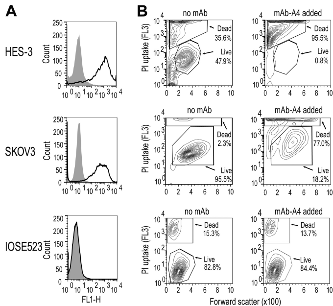
Figure 1. Binding and cytotoxicity of mAb-A4 to cancer and normal and human embryonic stem cell lines. A , mAb-A4 binding to HES-3 (top), SKOV3 (middle), and IOSE523 (bottom). Histograms of negative control (filled) were overlaid with mAb-A4-treated samples (black line). B , mAb-A4 cytotoxicity against HES-3 (top), SKOV3 (middle), and IOSE523 (bottom), showing untreated controls (left column) and mAb-treated samples (right column). Contour plots of forward scatter versus FL3 PI uptake were gated for live and dead populations based on the untreated cells. The data shown are representative of three biological replicates.
