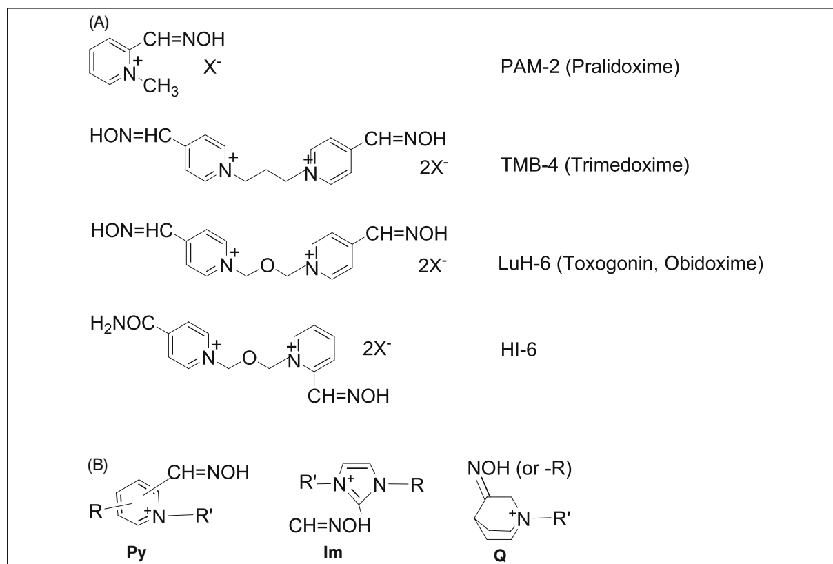
Figure 1 (A) Structure of conventional antidotes ( X^- is an anion) used in the treatment of OP poisoning and (B) general structure of quaternary pyridinium (Py), imidazolium (Im) and quinuclidinium (Q) derivatives described in reference (7)
