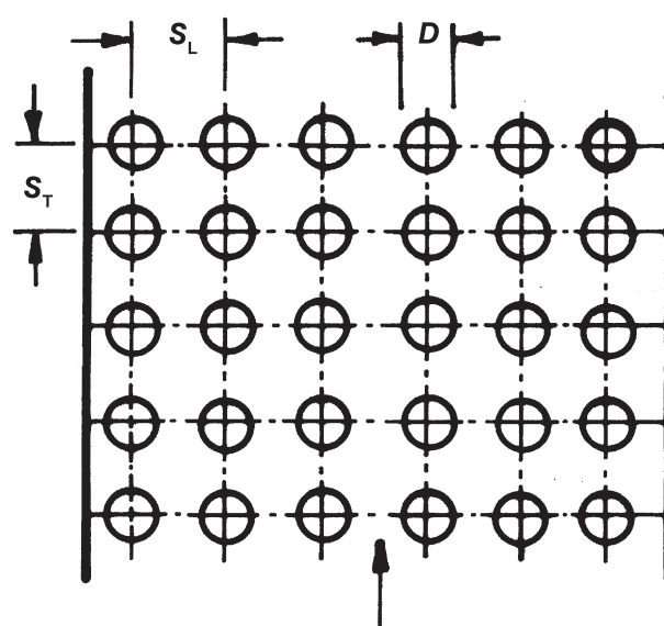
Fig. 2 – Arrangement of tube bank in the column. S_L = longitudinal pitch, S_T = transverse pitch. D = tube diameter, S_T = S_L = 2D , D = 8 \text{ mm}
