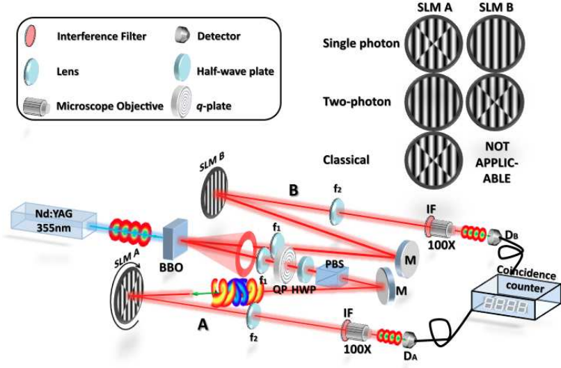
FIG. 1: Setup used for the two quantum-regime experiments. A Nd:YAG laser with average power of 150 mW at 355 nm pumps a nonlinear crystal of \beta -barium borate (BBO) cut for degenerate type-I non-collinear phase matching which emits OAM-entangled H -polarized photon pairs at 710 nm (see Ref. [18] for details). The photons of each pair are split in arms A and B , respectively. Legend of the main components (see also graphic symbol legend in the upper-left inset): f_1 , f_2 - lenses for beam control; QP - q -plate; HWP - half-wave plate; PBS - polarizer; M - mirror; SLM A and SLM B - spatial light modulators; IF - interference filter for bandwidth definition; 100X - microscope objectives for fiber coupling; D_A , D_B - photon detectors. In the classical-regime experiment, the optical line is the same as arm A . Top-right inset: computer-generated hologram patterns displayed on the two SLMs in the three experiments.
