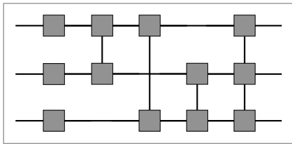
Figure 5: The evolution stage of an exponential (highly-entangling) measurement procedure involving N = 3 quantum systems. The query complexity scales exponentially with the number of quantum systems, that is, Q = 2^N - 1 .
