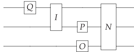
Figure 2: An example of a quantum network consisting of single ( Q, P, O ) and many-body ( I, N ) quantum gates.
