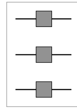
Figure 3: The evolution stage of a linear (non-entangling) measurement procedure involving N = 3 quantum systems. The query complexity is linear in the number of quantum systems, that is, Q = N .
