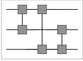
Figure 4: The evolution stage of a two-body (entangling) measurement procedure involving N = 3 quantum systems. The query complexity scales quadratically with the number of quantum systems, that is, Q = \frac{1}{2}N(N - 1) .
