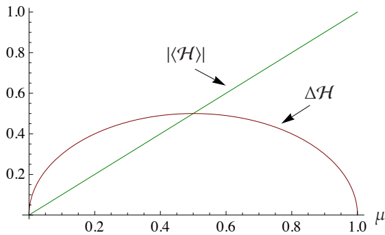
Figure 6: The expectation value of the generator \mathcal{H} above the ground state versus the standard deviation of the generator \mathcal{H} as a function of \mu [with \|\mathcal{H}\| = 1 a.u.].
