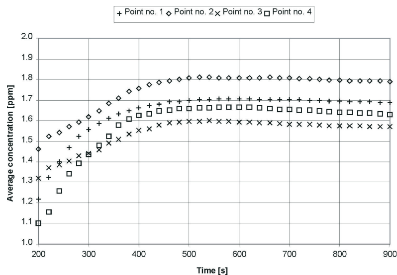
Figure 5. Tracer gas distribution within the employees' breathing zone
