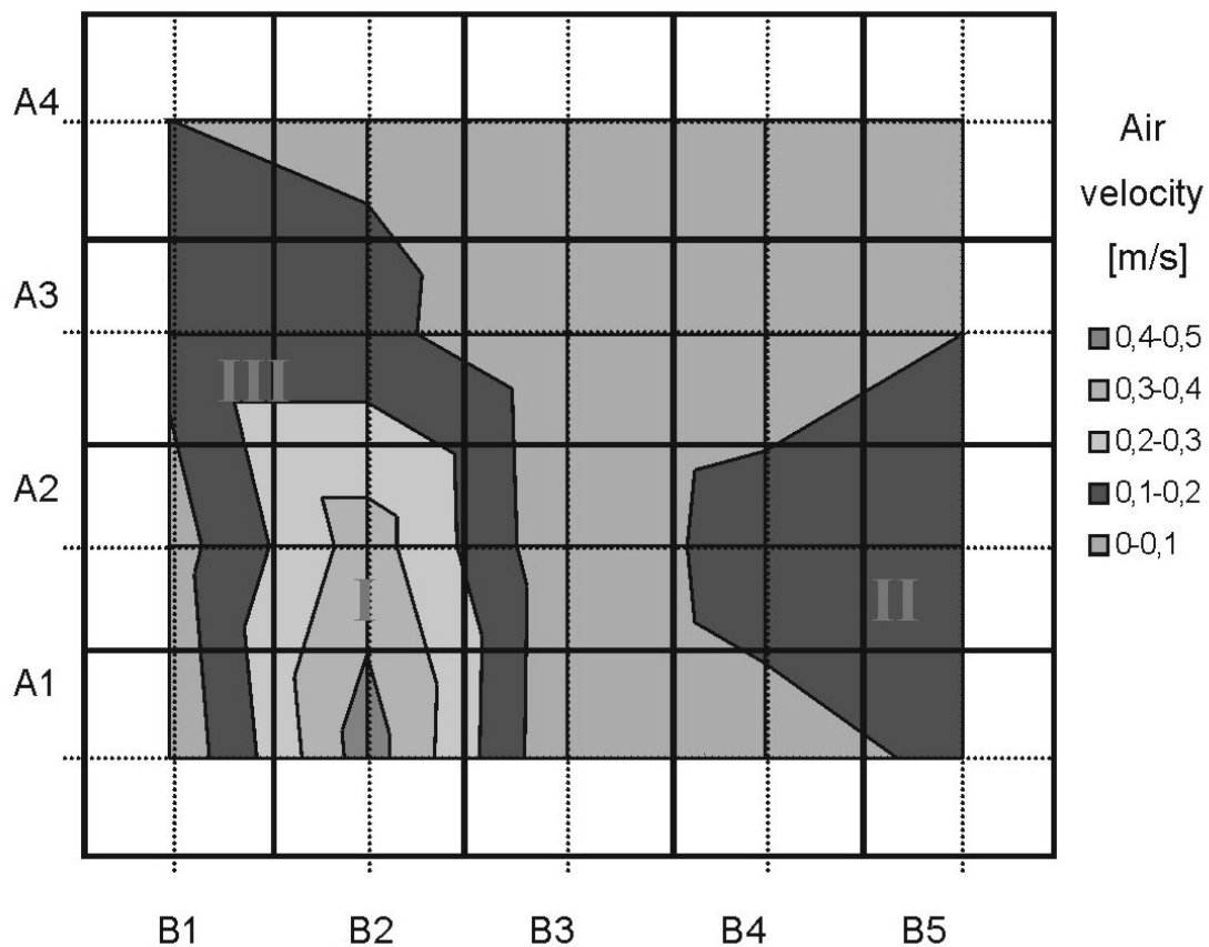
Figure 4. Air velocity distribution at the dimension of 1.5 m above the working room floor Slika 4. Distribucija brzine zraka na 1,5 m iznad poda radne prostorije
