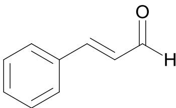
Figure 1. Structure of trans -cinnamaldehyde or cinnamaldehyde.
