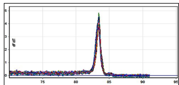
Fig.2: Sequencing analysis of R376W mutation.
