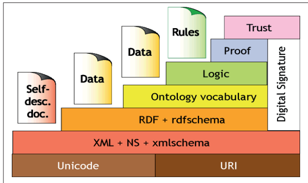
Figure 1. Semantic web architecture
