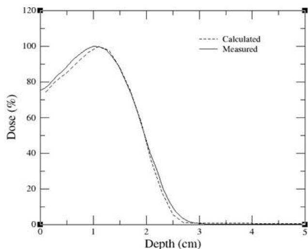
Figure 2: Comparison of measured 5 MeV and calculated 5.9 MeV PDD curves for 10 × 10 cm 2 field size and 100 SSD.
