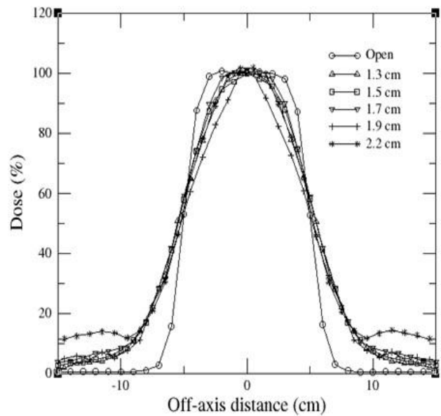
Figure 6: Dose profile of 5 MeV electron beam for 10 \times 10 \text{ cm}^2 , open field and with different thicknesses of spoiler.
