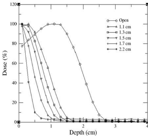
Figure 5: PDD curves for 5 MeV electron beam for 20 \times 20 \text{ cm}^2 , open field and different thicknesses of spoiler.
