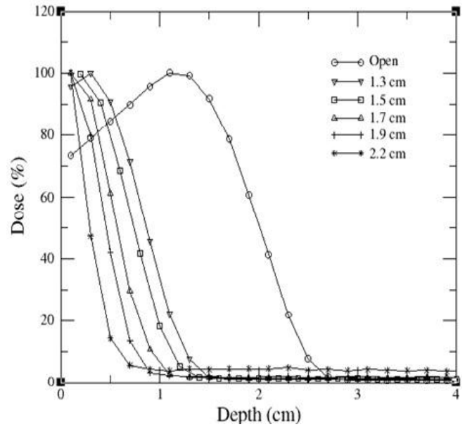
Figure 4: PDD curves for 5 MeV electron beam for 10 \times 10 \text{ cm}^2 , open field and different thicknesses of spoiler.
