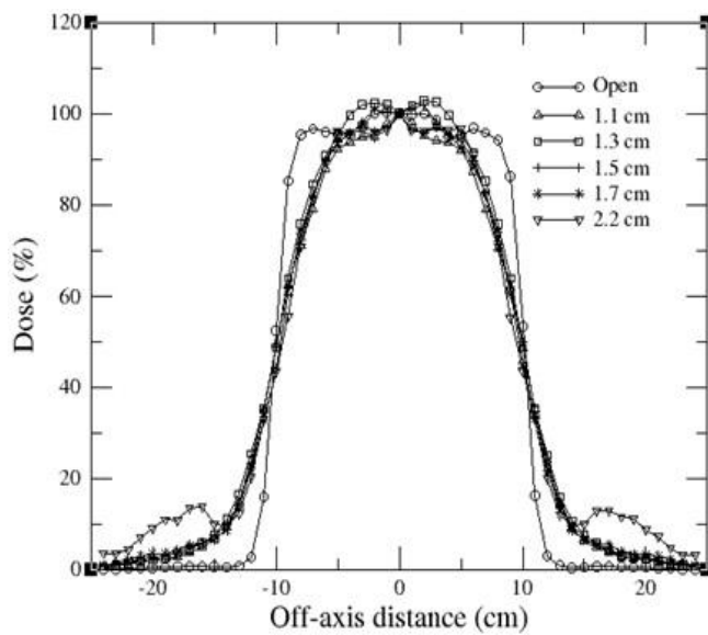
Figure 7: Dose profile of 5 MeV electron beam for 20 \times 20 \text{ cm}^2 , open field and with different thicknesses of spoiler.
