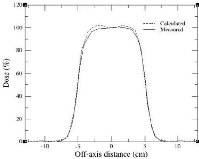
Figure 3: Comparison of measured 5 MeV and calculated 5.9 MeV dose profile curves for 10 \times 10 \text{ cm}^2 field size and \text{SSD}=100 \text{ cm} .
