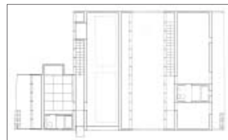
FIG. 12 KAZUYO SEJIMA & RYUO NISHIZAVA: M-HOUSE, TOKIO, 1997
