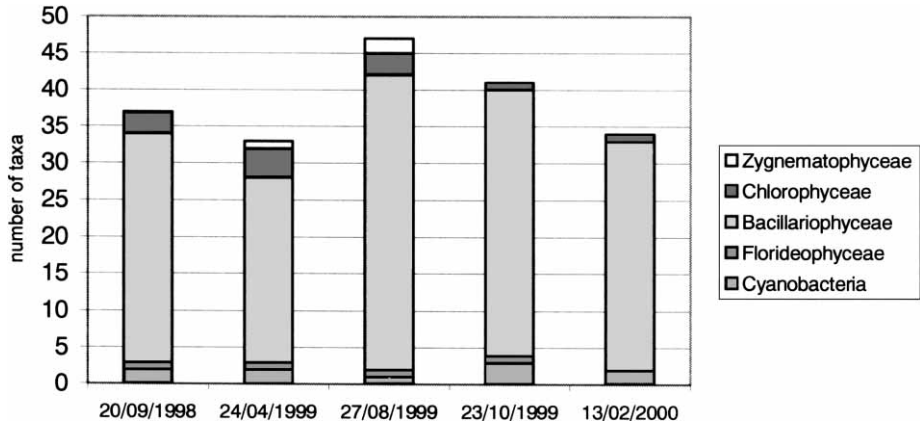
Fig. 2. Number of species from a travertine barrier of the Krka River during the investigation.
