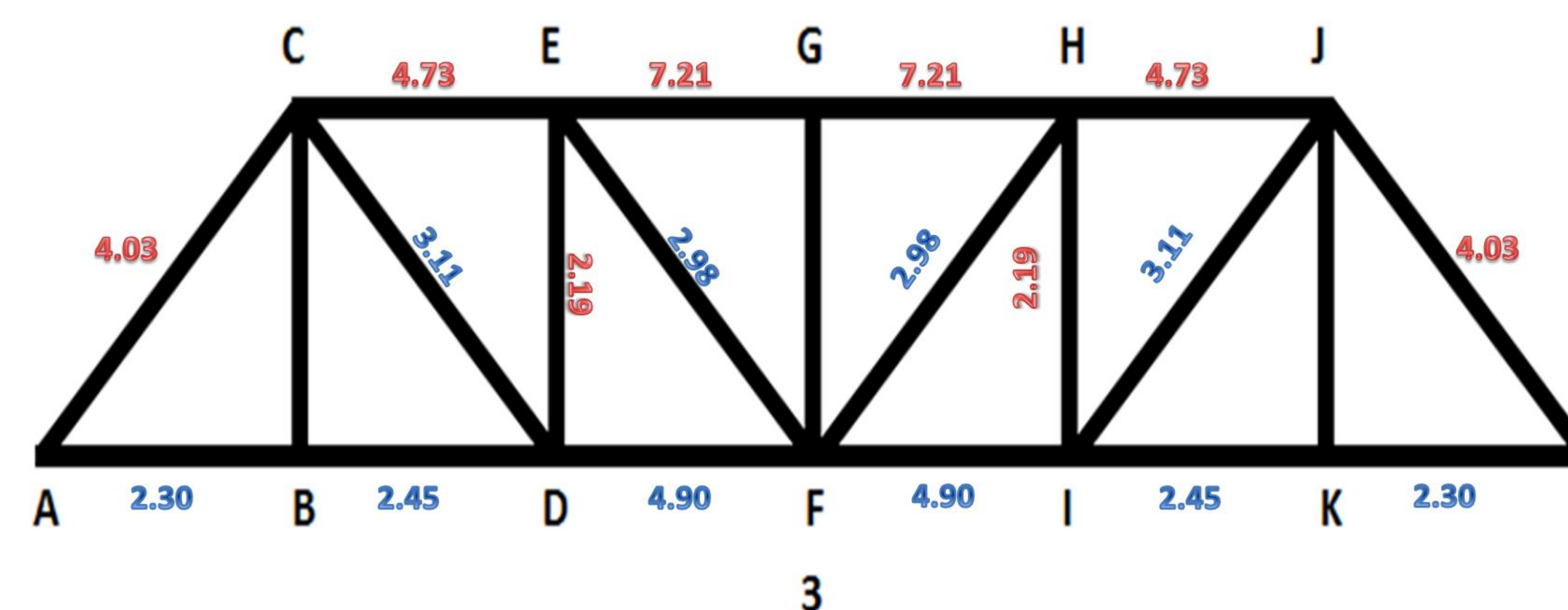
Fig. 3 Forces in Pratt bridge with load in position 3
