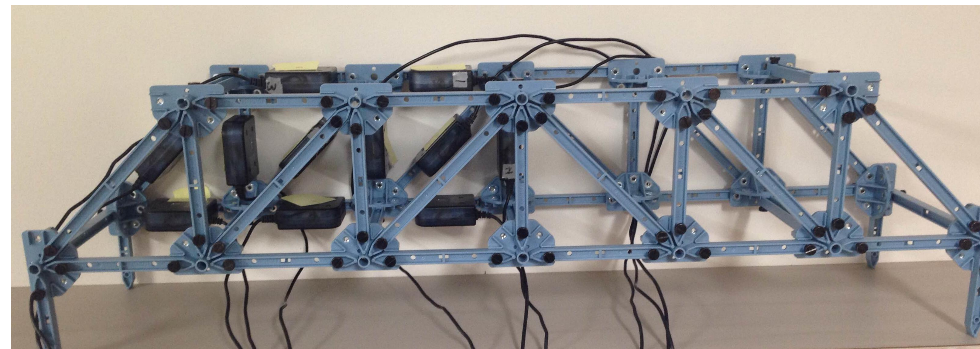
Fig. 2 Howe bridge model
