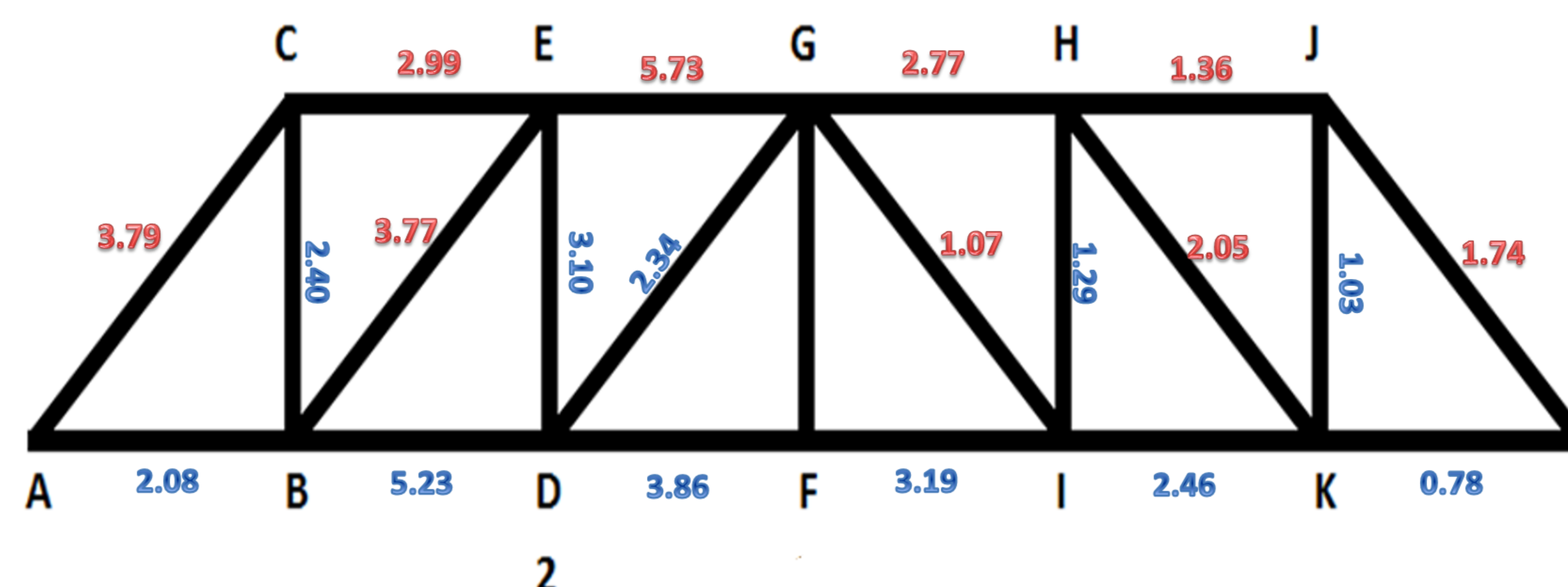
Fig. 4 Forces in Howe bridge with load in position 2
