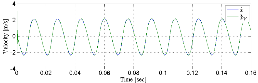
Figure 10. Comparison of velocity, measured \dot{x}(t) and observed \hat{\dot{x}}_v(t) .
