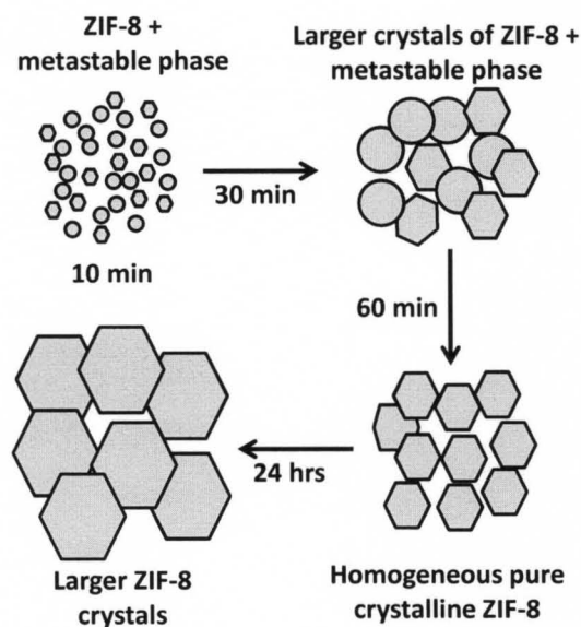
Figure 6.11. Proposed formation pathway of ZIF-8 as a function of synthesis time.
