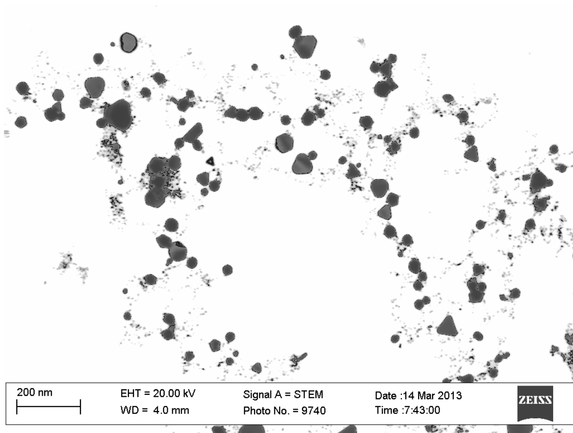
FIGURE 39 - STEM Image 02
