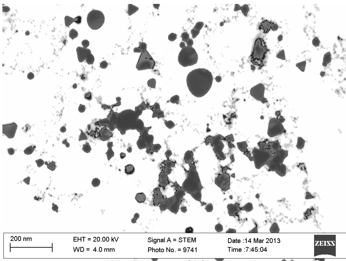
FIGURE 40 - STEM Image 03
