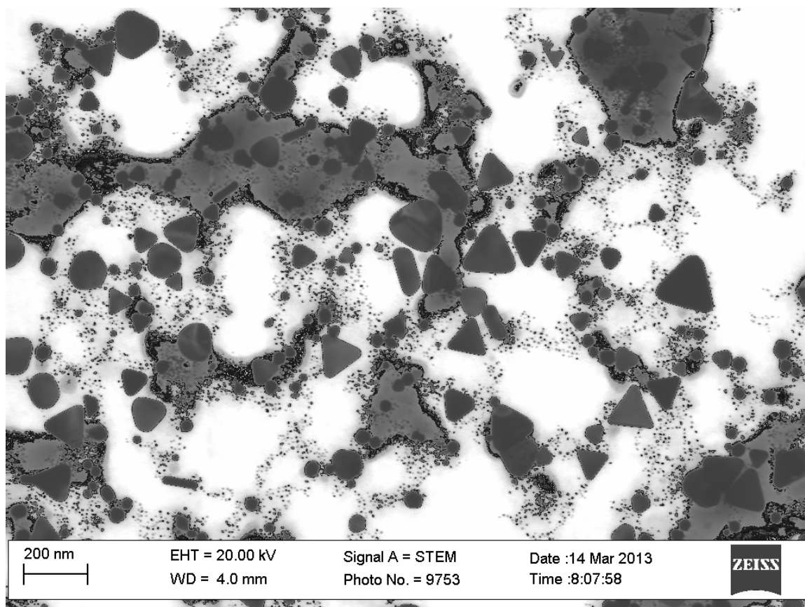
FIGURE 41 - STEM Image 04
