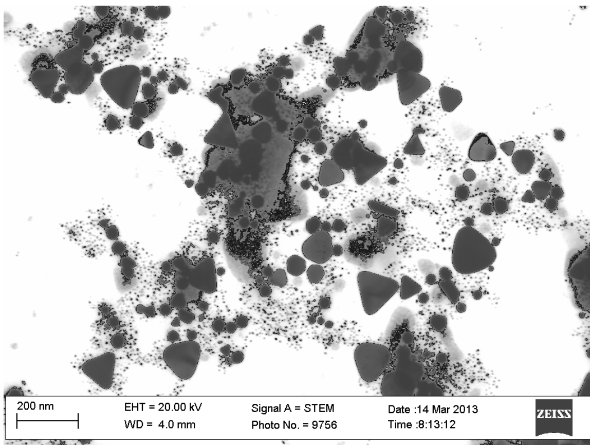
FIGURE 43 - STEM Image 06
