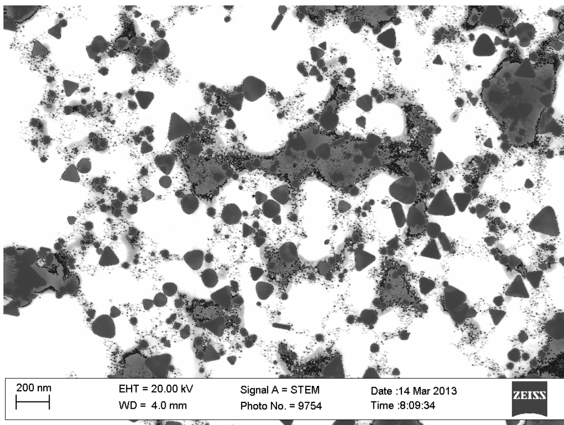
FIGURE 42 - STEM Image 05
