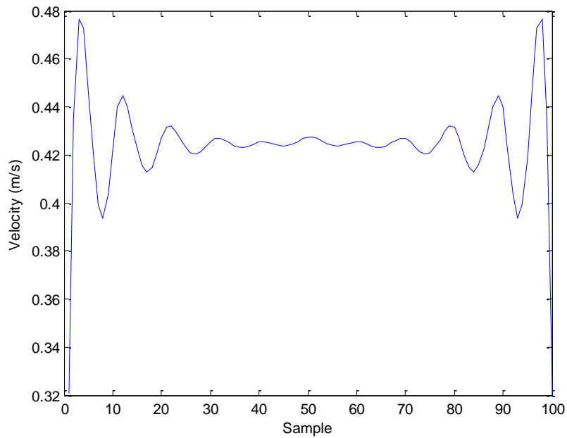
FIGURE 22 - Linear Velocity of the Differential Drive Robot
