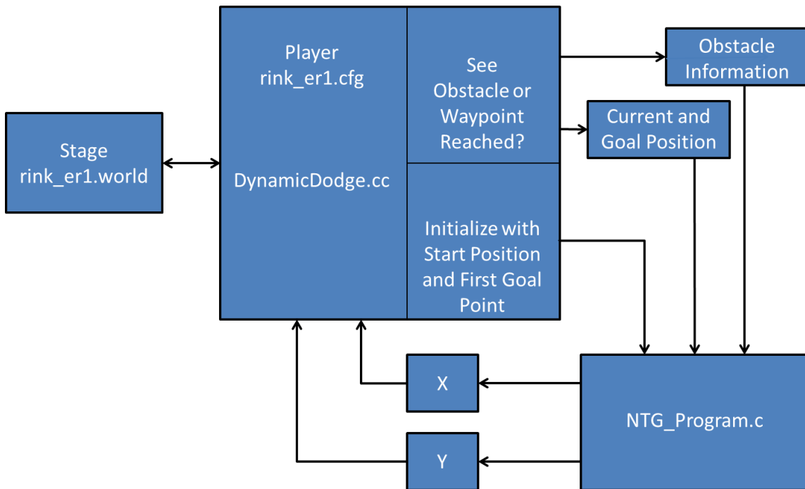
FIGURE 24 - Player/Stage/NTG Software Flowchart
