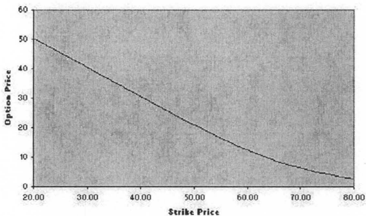
Figure 4.14 Graph of option price as a function of strike price, K , with an asset price, S_0 , of $70 and volatility of 30%.
