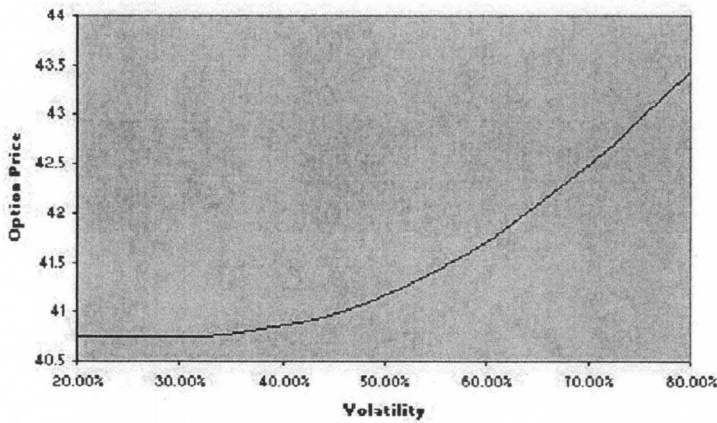
Figure 4.9 Graph of option price as a function of volatility, with a current asset price, S_0 , of $90.
