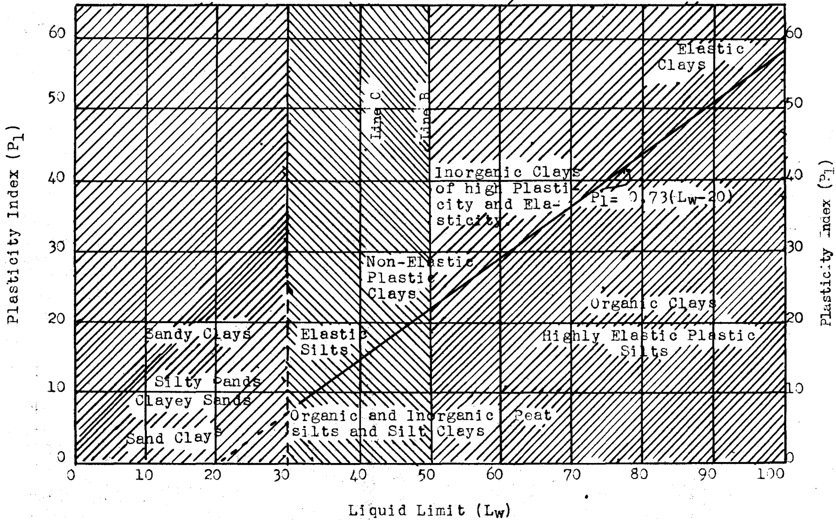
FIG. 12 - PLASTICITY CHART
