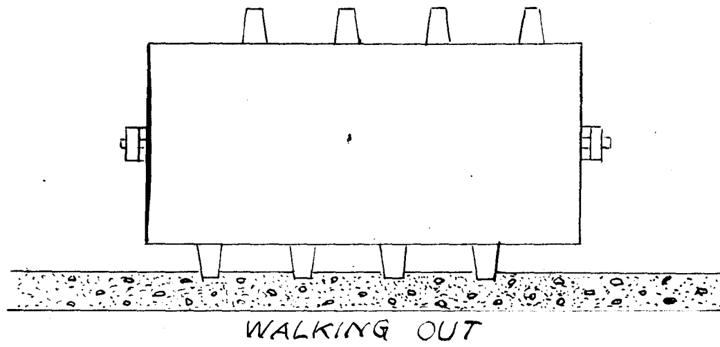
FIG 33 SHEEPSFOOT ROLLER ACTION ON COM- PACTING A FILL
