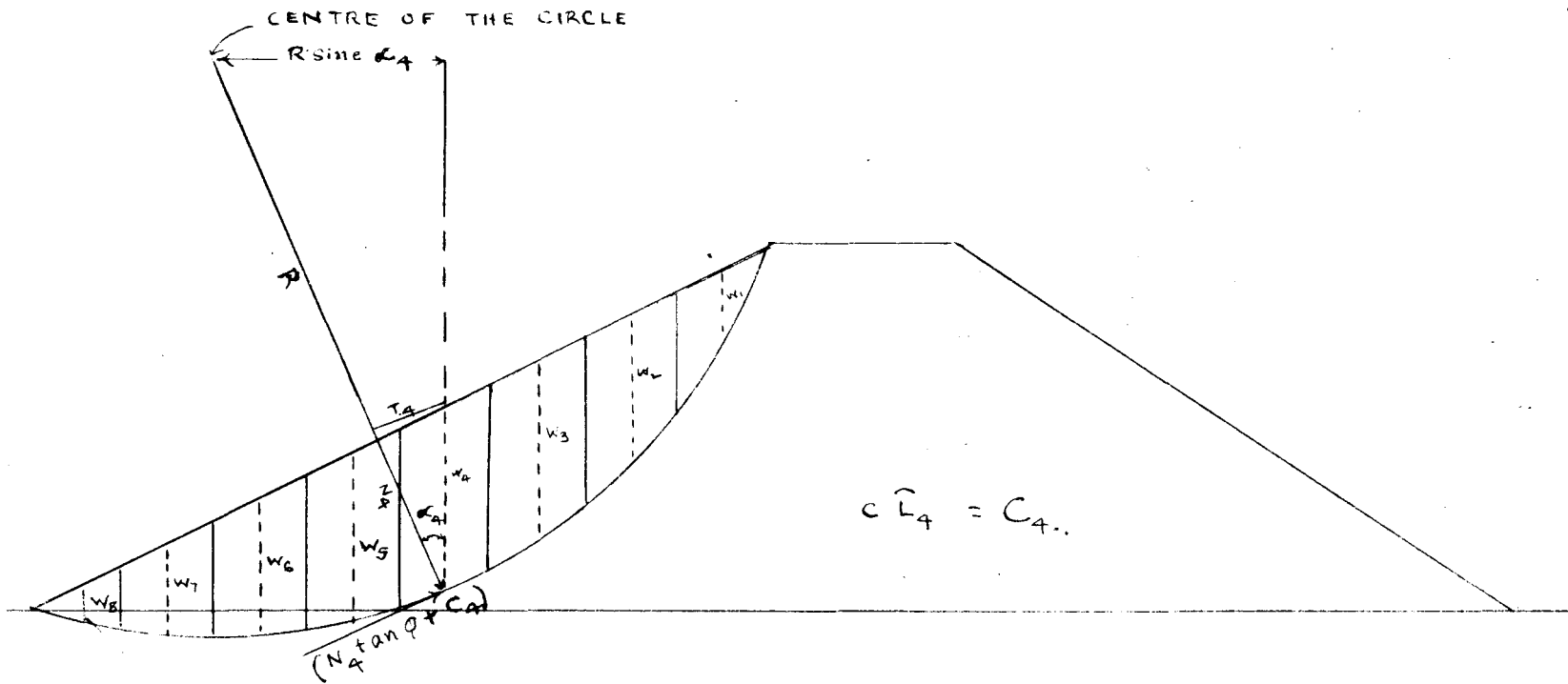
FIG. 17 DERIVATION OF FORMULA TO FIND FACTOR OF SAFETY (F.S). \bar{L}_4 = Length of arc of slice 4
