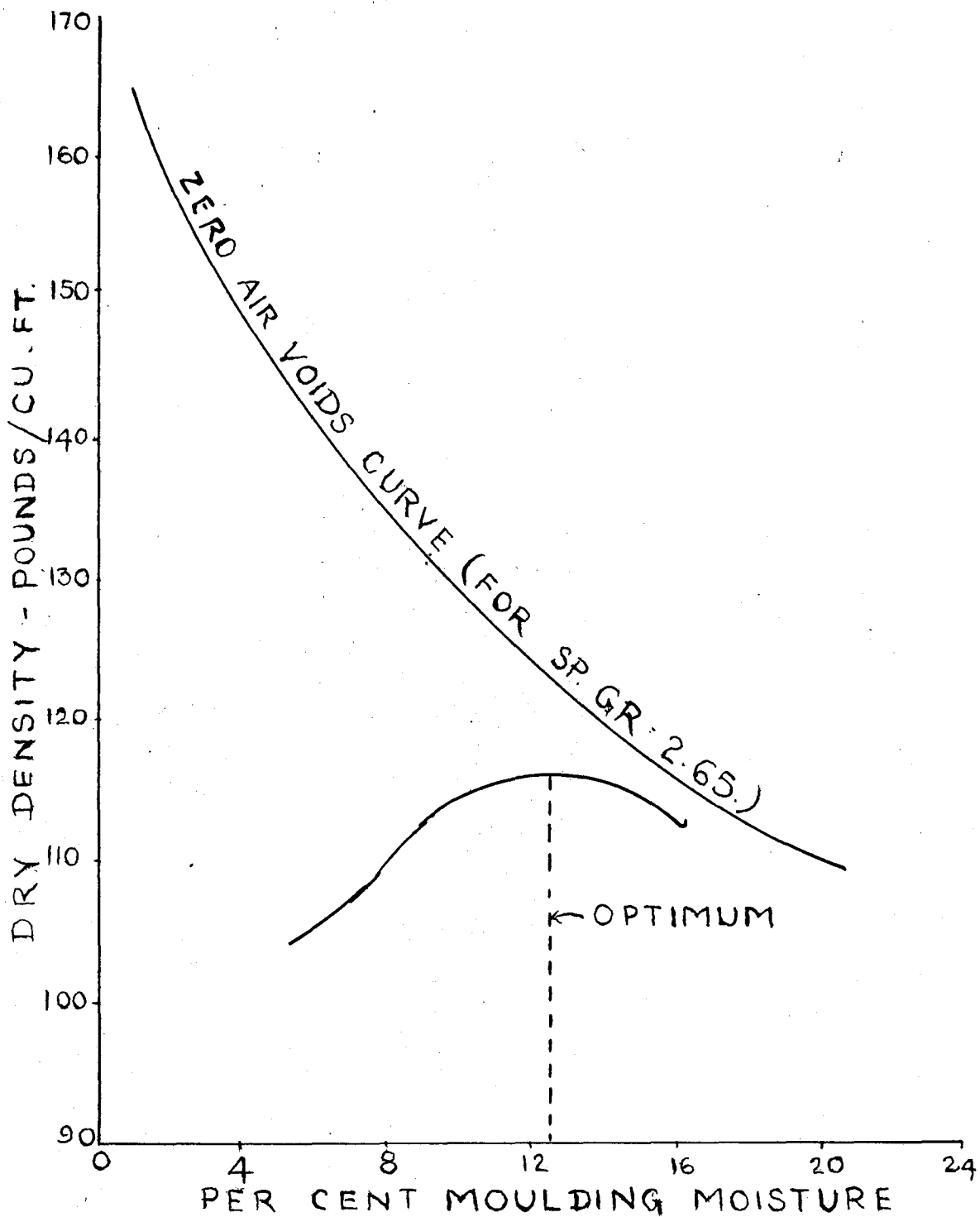
FIG.30 SAMPLE PROCTER SHEET FOR EARTH COMPACTION
