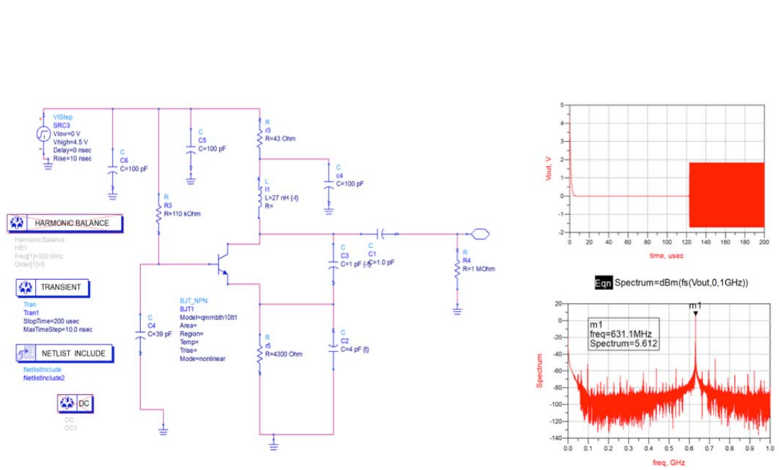
Figure 89. Discrete Colpitts oscillator schematic and output signal with spectrum.
