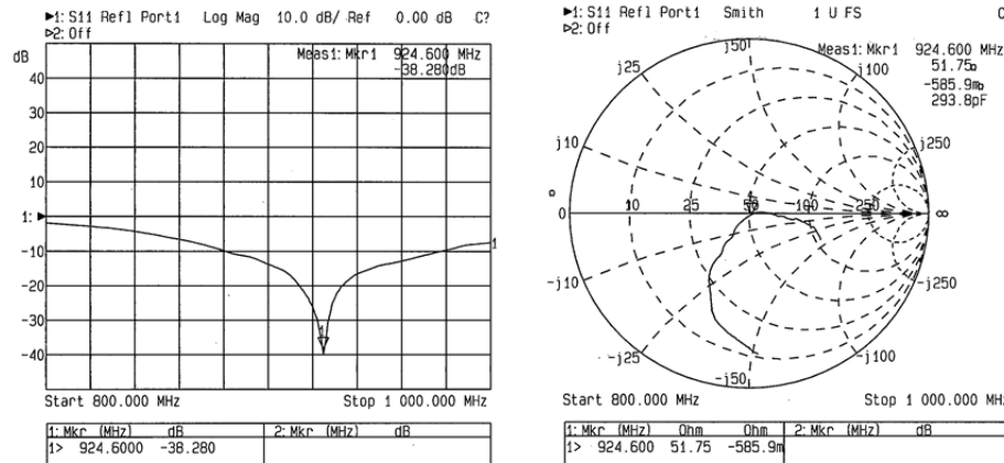
Figure 37. Forward transmission parameters of folded dipole antenna showing resonant frequency and impedance at resonance.
