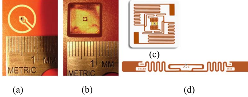
Figure 11. (a) Impinj “Button” antenna, (b) HF (3 – 30 MHz) antenna, (c) Alien Technology “Square Antenna”, 22.5 mm x 22.5 mm, (d) Alien Technology “Squiggle” antenna, 95 mm x 8.2 mm.
