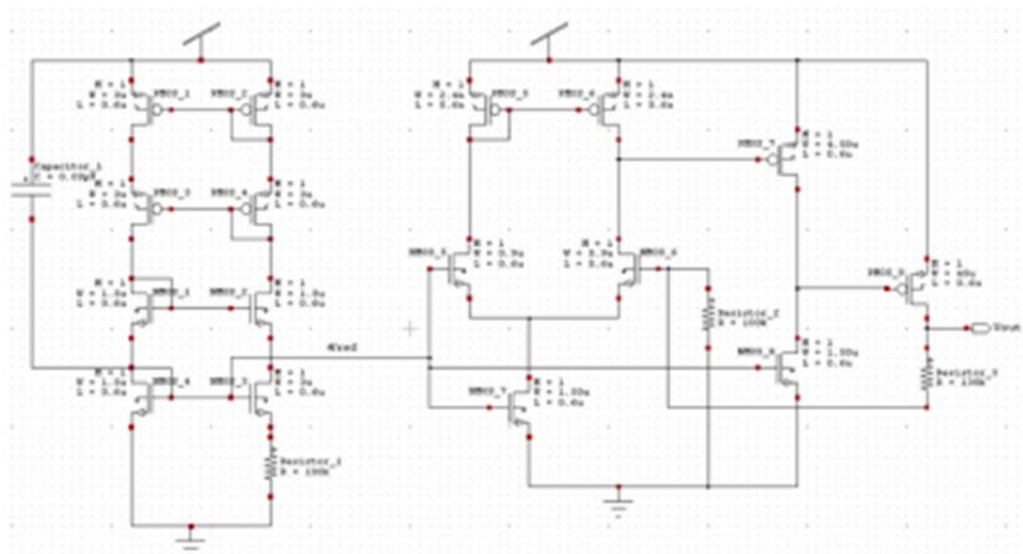
Figure 141. Voltage regulator with reference.
