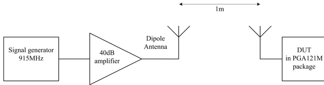
Figure 114. Test setup for radiated RF-to-DC conversion: circuit in PGA package.
