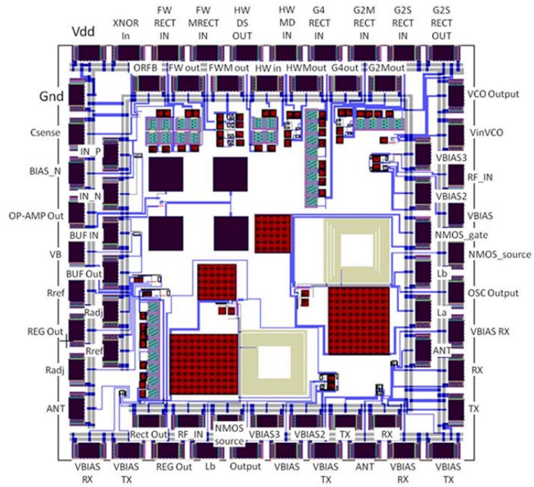
Figure 103. ASIC pin layout.
