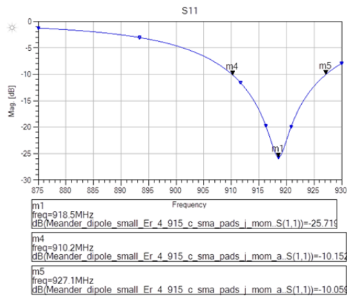
Figure 56. Return Loss: Antenna (a)
