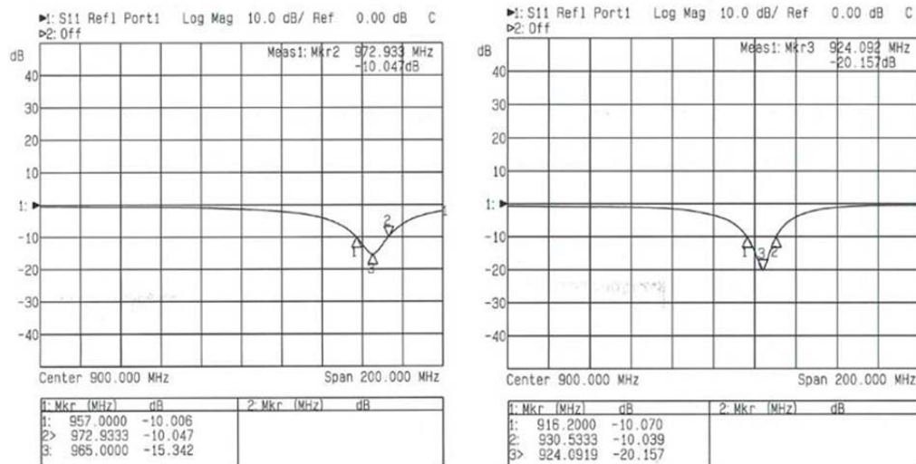
Figure 57. Return Loss: Antenna (a) Antenna (d).
