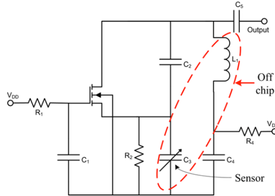
Figure 145. Colpitts oscillator circuit schematic.
