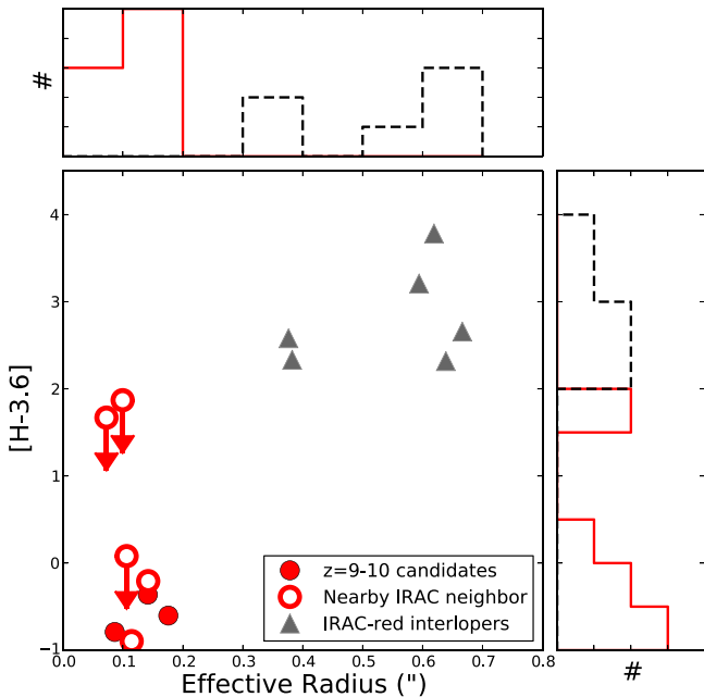
Figure 4. z \sim 9 – 10 galaxy candidates from Oesch et al. (2013b, 2014) and the interlopers to the z \sim 9 – 10 selection where the H - [3.6] or H - [4.5] criterion is not applied. Those objects with close companions in the IRAC 3.6 \mu\text{m} images (see Figure 4 in Oesch et al. 2013b and Figure 2 in Oesch et al. 2014) are indicated with open circles and with arrows where lower limits on the flux measurements are relevant. The effective radii ( r_e ) and H - 3.6 colors for z \sim 9 – 10 galaxy candidates from Oesch et al. (2014, red circles) and interlopers to a z \sim 9 – 10 selection (gray triangles) when no H - [3.6] or H - [4.5] criterion is applied. The z \sim 9 – 10 galaxies and the lower-redshift interlopers separate well in both their measured H - [3.6] colors and sizes. This suggests that the sizes of z \sim 9 – 10 candidates could serve as an alternate constraint on the high-redshift nature of z \sim 9 – 10 candidates where no Spitzer /IRAC data are available (e.g., as with the BORG program).
