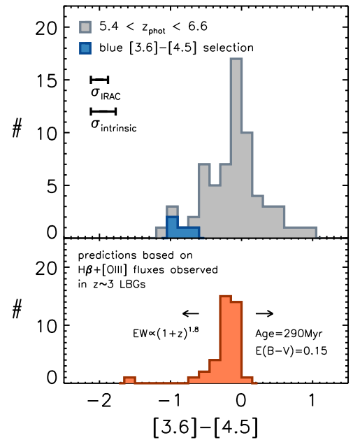
Figure 6. Top panel: the [3.6] - [4.5] color distribution (gray histogram) of sources with photometric redshifts (from the HST photometry) within the redshift range z \sim 5.4 - 6.6 (68% confidence) where [\text{O III}] contributes to the 3.6 \mu\text{m} flux, while \text{H}\alpha contributes to the 4.5 \mu\text{m} flux. Sources that satisfy our ultra-blue IRAC selection criterion (Equation (2)), but prefer a z < 6.6 are indicated with the blue histogram (note that for a few sources the very blue [3.6] - [4.5] colors are not significant). The upper error bar on the left side of the panel indicates the scatter in the [3.6] - [4.5] color distribution due to photometric uncertainty in the IRAC bands. The lower error bar indicates the intrinsic scatter, as calculated from the observed scatter and the simulated IRAC uncertainties. Bottom panel: the predicted [3.6] - [4.5] color distribution (orange histogram) using the [\text{O III}] and \text{H}\beta EWs as measured by Schenker et al. (2013b) and Holden et al. (2014) in z \sim 3 LBGs with the MOSFIRE spectrograph. We predict the [3.6] - [4.5] color assuming Case B recombination and a flat continuum in f_\nu . Evolution of the EW strength as a function of redshift (e.g., Smit et al. 2014) will broaden the [3.6] - [4.5] color distribution and at the same time shift the median color of the distribution to bluer values as indicated by the left black arrow on the panel. The right black arrow indicates the shift in [3.6] - [4.5] color when we assume a somewhat more evolved stellar population with an age of 290 \text{ Myr} and a dust content of E(B - V) = 0.15 (see Section 4.2 for details).
