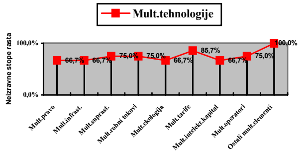
Graph 9. Indirect growth rates of multimodal technologies in relation to other elements of multimodal model
