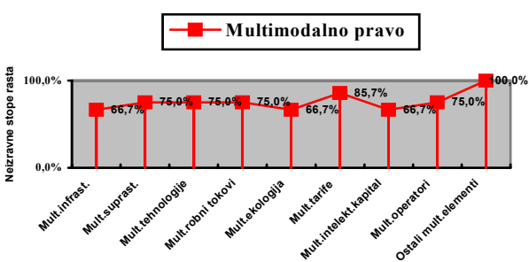
Graph 3. Indirect growth rates of multimodal law in relation to other elements of multimodal model
