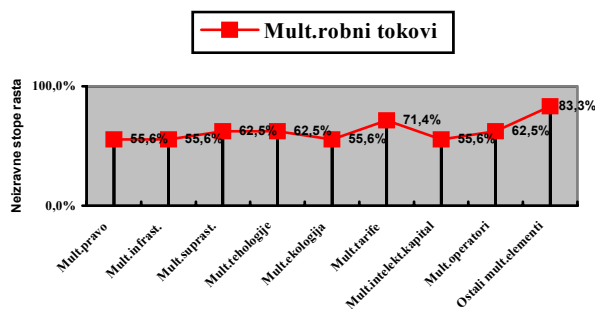
Grafikon 11. Neizravne stope rasta multimodalnih robnih tokova u odnosu na ostale elemente multimodalnog modela Graph 11. Indirect growth rates of multimodal commodity flows in relation to other elements of multimodal model
