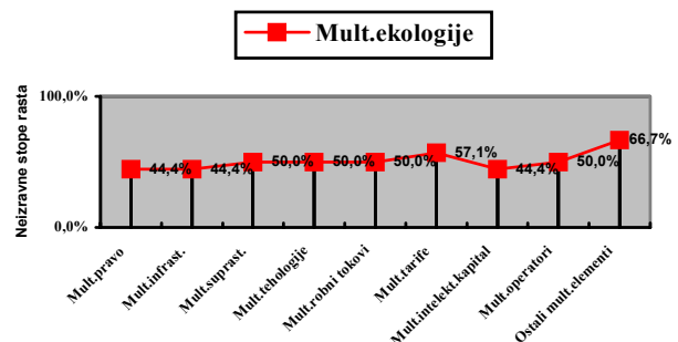
Grafikon 13. Neizravne stope rasta multimodalne ekologije u odnosu na ostale elemente multimodalnog modela Graph 13. Indirect growth rates of multimodal ecology in relation to other elements of multimodal model
