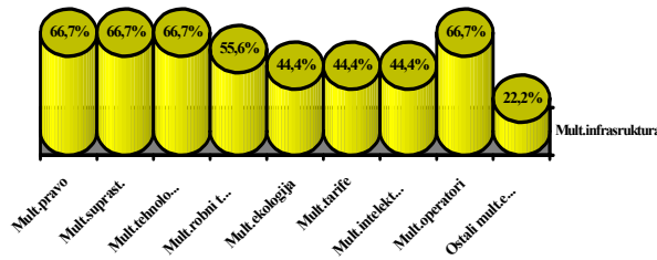
Graph 6. Indirect growth rates of other elements of multimodal model in relation to multimodal infrastructure
