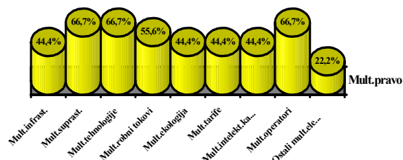
Graph 4. Indirect growth rates of other elements of multimodal model in relation to multimodal law
