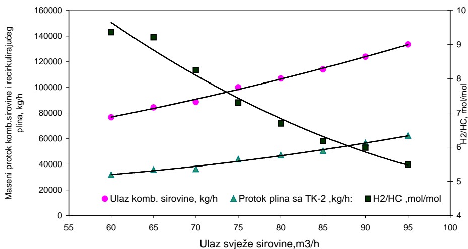
Slika 5: Ovisnost protoka kombinirane sirovine i recirkulirajućeg plina te omjera H_2/HC o protoku svježe sirovine Figure 5: Dependence of the combined charge and recycle gas flow and the H_2/HC ratio on the fresh charge flow
