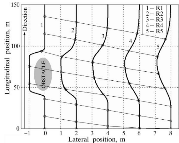
Fig. 11 Robots trajectories in x - y plane
