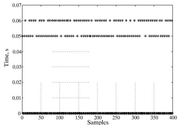
Fig. 4 Calculation time of control action of the I/O GPC for the in-
