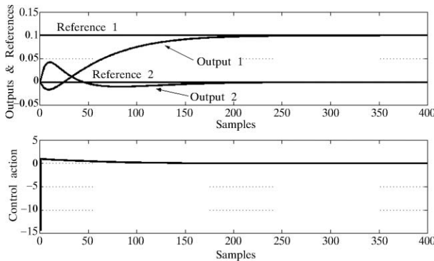
Fig. 2 Control of an inverted pendulum using state space GPC
