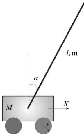
Fig. 1 Inverted pendulum
