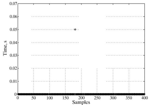
Fig. 3 Calculation time of control action of the state space GPC for the inverted pendulum
