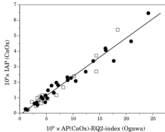
Fig. 3. Correlation between ionic activity products (IAP(CaOx)) and AP(CaOx)-EQ2-indexes (Ogawa) for patients (●) and controls (□); correlation coefficient is r=0.97 , p<0.0001 .
