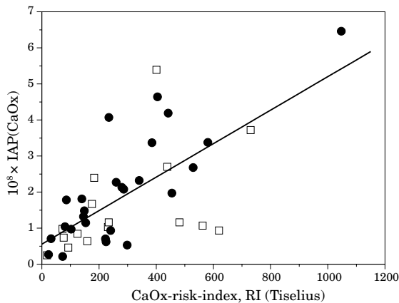
Fig. 2. Correlation between ionic activity products (IAP(CaOx)) and CaOx-risk-indexes, RI (Tiselius) for patients (●) and controls (□); correlation coefficient is r=0.68 , p<0.0001 .
