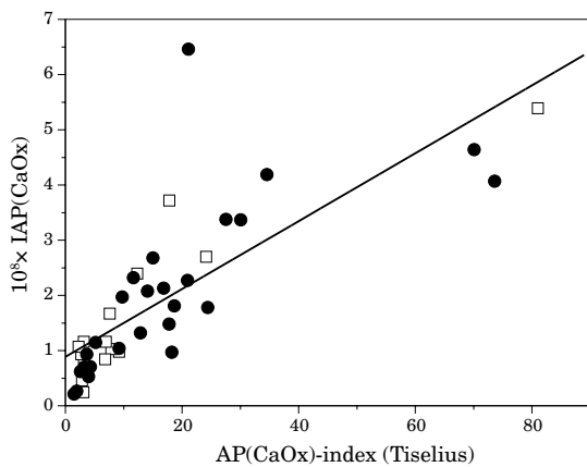
Fig. 1. Correlation between ionic activity products (IAP(CaOx)) and AP(CaOx)-indexes (Tiselius) for patients (●) and controls (□); correlation coefficient is r=0.78 , p<0.0001 .
