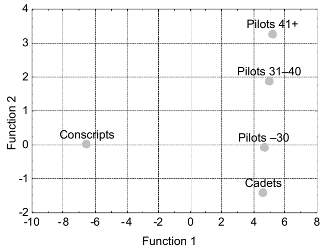
Fig. 1. Position of cadets, pilots of different age groups and conscripts with regard to the first two discriminant functions.
