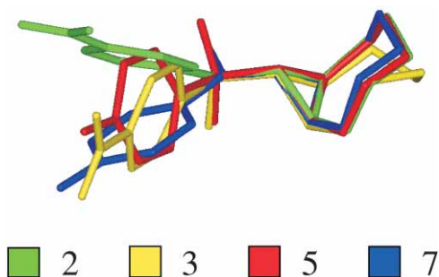
Figure 5. Superposition of solid state conformations of azirines 2 , 3 , 5 and 7 .
