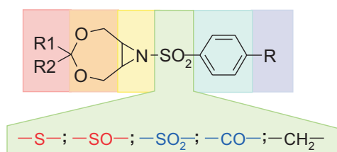
Figure 1. Variation of sulphonyl moiety of N -aryl-1a,2,6,6a-tetrahydro-1H,4H-[1,3]dioxepino[5,6- b ]azirine.
