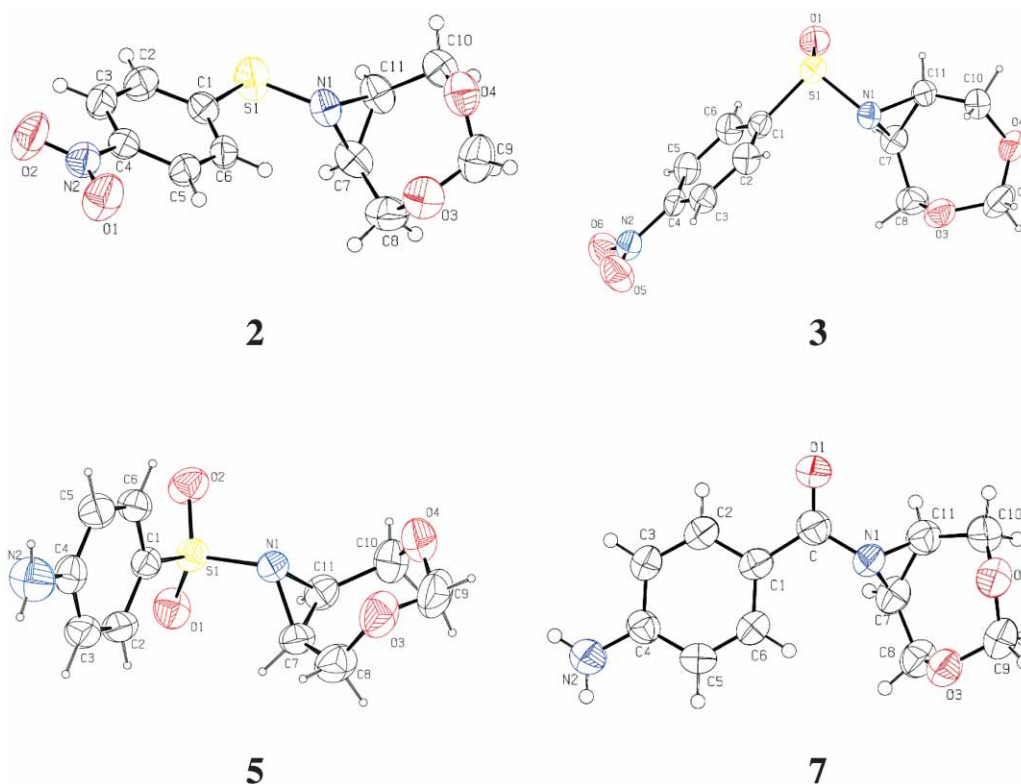
Figure 2. TEP of 2 , 3 , 5 and 7 crystal structures with atomic numbering (Ellipsoids drawn at 50 % probability level).
