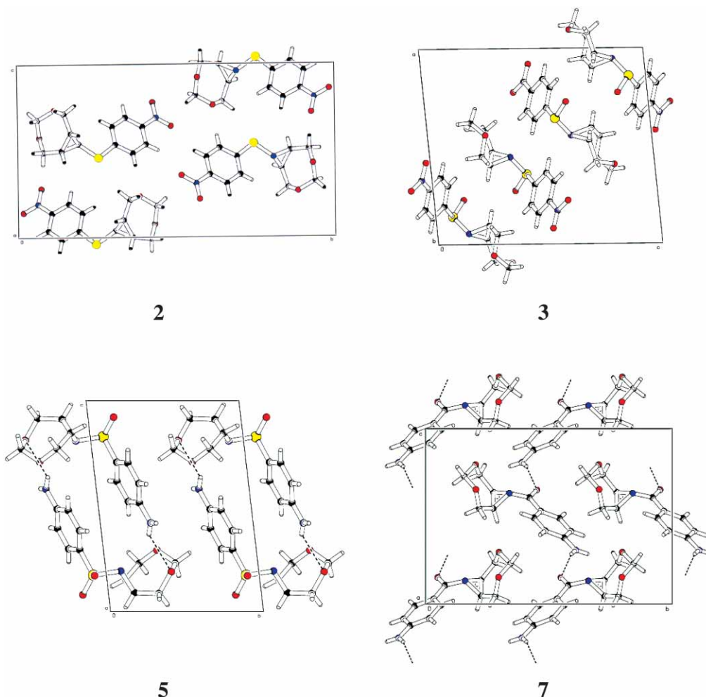
Figure 4. Crystal packing of azirines 2 , 3 , 5 and 7 .
