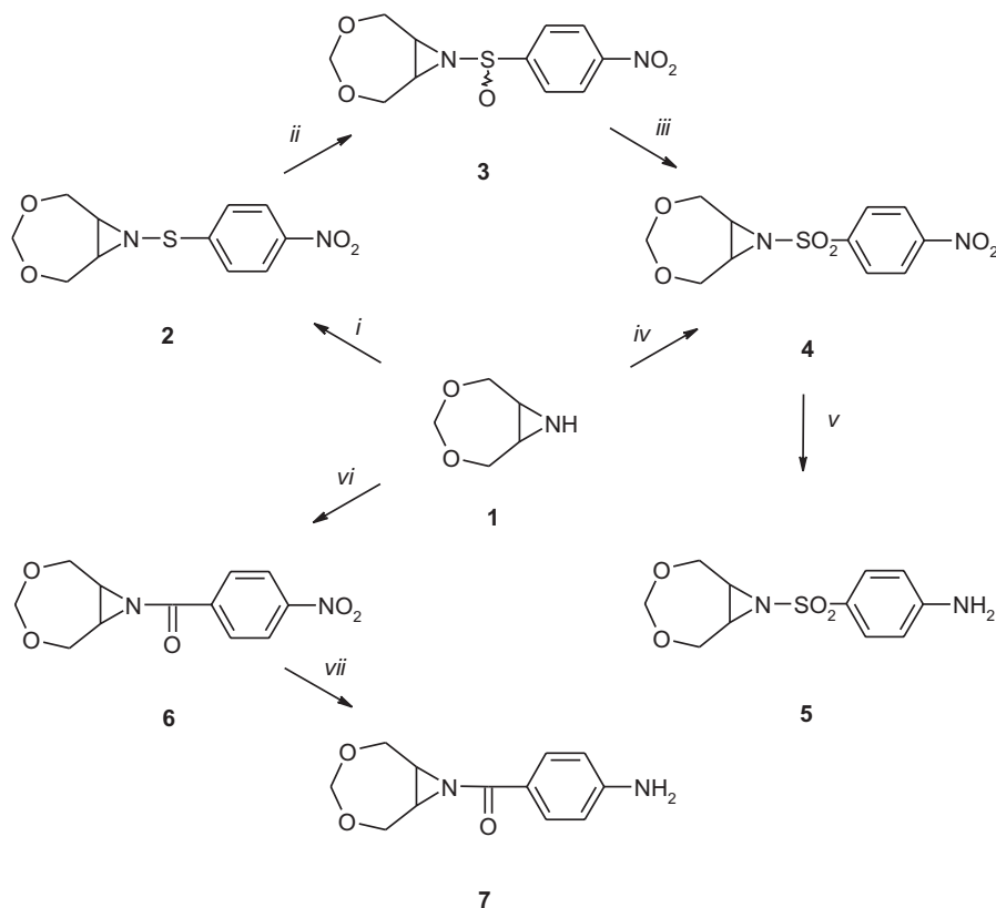
Scheme 1. Synthesis of nitro- and aminoaryl-azirines 2-7 . Reagents and conditions: i , 4-nitrobenzenesulphenyl chloride/pyridine/ \text{CH}_2\text{Cl}_2 , r.t., 30 min. under \text{N}_2 ; ii , m -CPBA/ \text{CH}_2\text{Cl}_2 , r.t., 2 h; iii , \text{KMnO}_4/\text{HOAc-EtOAc} , 5 °C; iv , 4-Nitrobenzenesulphonyl chloride/pyridine/ \text{CH}_2\text{Cl}_2 , 0 °C, 1 h 1 ; v , \text{H}_2/5\% \text{ Pd/C} , EtOAc, 1 bar, r.t., 3 h; vi , 4-nitrobenzoyl chloride/pyridine/ \text{CH}_2\text{Cl}_2 , refl., 1 h 1 ; vii , \text{H}_2/5\% \text{ Pd/C} , methanol, 3 bar, r.t., 3 h.
