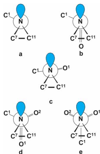
Figure 3. Solid state conformations: Sulphonyl-, sulphinyl-, and carbonylaziridine moieties of 2 , 3 , and 7 adopt conformations a , b and c , while sulphonylaziridine moiety of 5 adopts only conformation d of the two possible ones, d and e .
