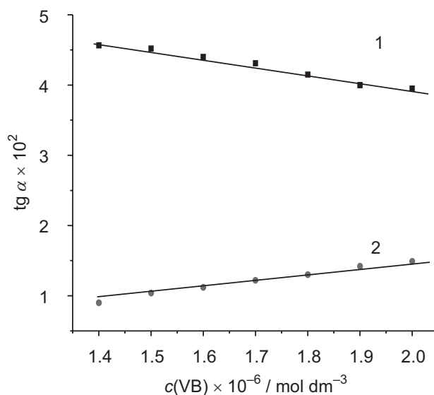
Figure 5. Dependence of the reaction rate of VB and \text{KBrO}_3 on VB concentration. 1 – indicating reaction (without \text{As}^{3+} ), 2 – inhibiting reaction (with \text{As}^{3+} ). Initial conditions: c(\text{HCl}) = 2.25 \times 10^{-2} \text{ mol dm}^{-3} , c(\text{KBrO}_3) = 5 \times 10^{-4} \text{ mol dm}^{-3} , c(\text{KCl}) = 0.1 \text{ mol dm}^{-3} , \gamma(\text{As}^{3+}) = 5 \times 10^{-7} \text{ g cm}^{-3} , t = 22 \pm 0.1 \text{ }^\circ\text{C} .
