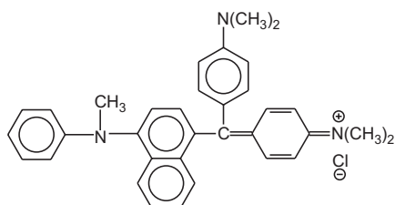
Figure 1. Chemical structure of Victoria Blue 4R. c.i. number 42563, c.i. name Basic Blue 8. (4-[(4-Dimethylamino-phenyl)-[4-(methyl-phenyl-amino)-naphthalene-1-yl]-methylene]-cyclohexa-2,5-dienylidene)-dimethyl-ammonium chloride.
