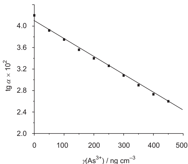
Figure 6. Calibration graph for \text{As}^{3+} determination. c(\text{HCl}) = 2.25 \times 10^{-2} \text{ mol dm}^{-3} , c(\text{KBrO}_3) = 5 \times 10^{-4} \text{ mol dm}^{-3} , c(\text{KCl}) = 0.1 \text{ mol dm}^{-3} , c(\text{VB}) = 2.0 \times 10^{-6} \text{ mol dm}^{-3} , t = 22 \pm 0.1 \text{ }^\circ\text{C} .
