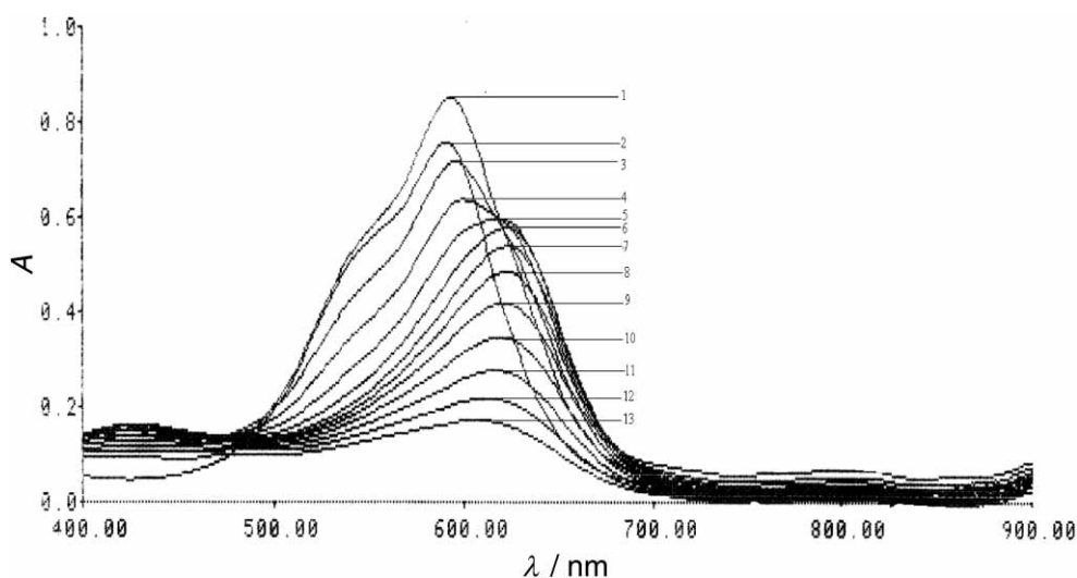
Figure 2. Absorption spectra of VB (1) and the indicating reaction mixture of VB and KBrO 3 (2–13) in acidic medium: effect of reaction time. Initial conditions: (1) c(\text{VB}) = 1.6 \times 10^{-6} \text{ mol dm}^{-3} , c(\text{HCl}) = 2.25 \times 10^{-2} \text{ mol dm}^{-3} , \varphi(\text{C}_2\text{H}_5\text{OH}) = 13 \% ; (2)–(13) c(\text{VB}) = 1.6 \times 10^{-6} \text{ mol dm}^{-3} , c(\text{HCl}) = 2.25 \times 10^{-2} \text{ mol dm}^{-3} , \varphi(\text{C}_2\text{H}_5\text{OH}) = 13 \% , c(\text{KBrO}_3) = 0.5 \times 10^{-3} \text{ mol dm}^{-3} , c(\text{KCl}) = 0.1 \text{ mol dm}^{-3} . Reaction time: (1) and (2) 0.5 min; (3) 1.0 min, (4) 1.5 min, (5) 2.0 min, (6) 2.5 min, (7) 3.0 min, (8) 3.5 min, (9) 4.0 min, (10) 4.5 min, (11) 5.0 min, (12) 5.5 min, (13) 6.0 min.
