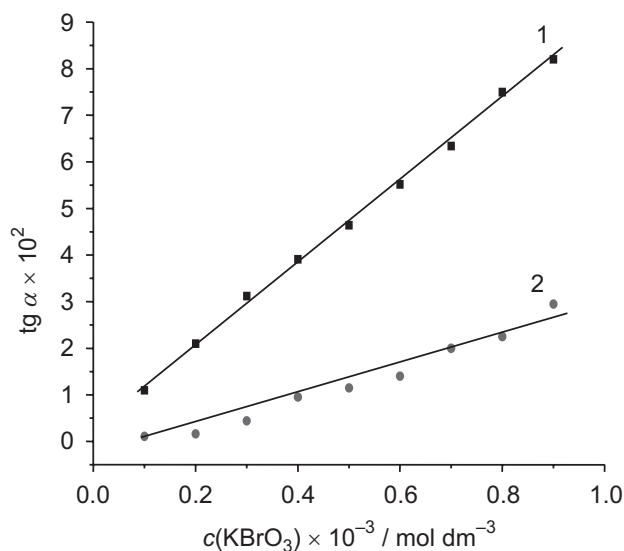
Figure 4. Dependence of the reaction rate of VB and \text{KBrO}_3 on \text{KBrO}_3 concentration. 1 – indicating reaction (without \text{As}^{3+} ), 2 – inhibiting reaction (with \text{As}^{3+} ). Initial conditions: c(\text{VB}) = 2.0 \times 10^{-6} \text{ mol dm}^{-3} , c(\text{HCl}) = 2.25 \times 10^{-2} \text{ mol dm}^{-3} , c(\text{KCl}) = 0.1 \text{ mol dm}^{-3} , \gamma(\text{As}^{3+}) = 5 \times 10^{-7} \text{ g cm}^{-3} , t = 22 \pm 0.1 \text{ }^\circ\text{C} .
