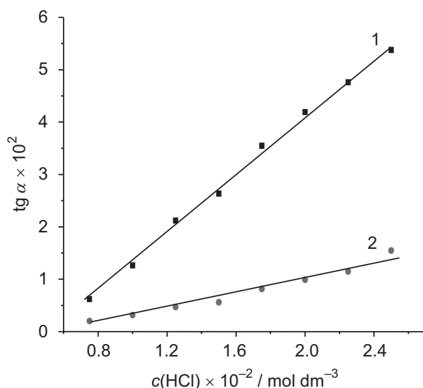
Figure 3. Dependence of the reaction rate of VB and \text{KBrO}_3 on HCl concentration. 1 – indicating reaction (without \text{As}^{3+} ), 2 – inhibiting reaction (with \text{As}^{3+} ). Initial conditions: c(\text{VB}) = 2.0 \times 10^{-6} \text{ mol dm}^{-3} , c(\text{KBrO}_3) = 5 \times 10^{-4} \text{ mol dm}^{-3} , c(\text{KCl}) = 0.1 \text{ mol dm}^{-3} , \gamma(\text{As}^{3+}) = 5 \times 10^{-7} \text{ g cm}^{-3} , t = 22 \pm 0.1 \text{ }^\circ\text{C} .
