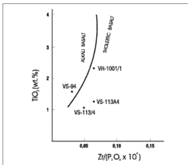
Fig. 13 \text{TiO}_2 vs. \text{Zr}/\text{P}_2\text{O}_5 diagram (WINCHESTER & FLOYD, 1976).
