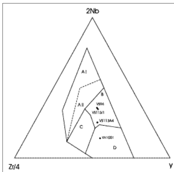
Fig. 17 Zr/4:2Nb:Y diagram (MESCHEDÉ, 1986). Legend: AI) within-plate alkali basalts; AII) within-plate alkali basalts and within-plate tholeiite; B) E-type MORB; C) within-plate tholeiite and volcanic-arc basalts; D) N-type MORB and volcanic-arc basalts.
