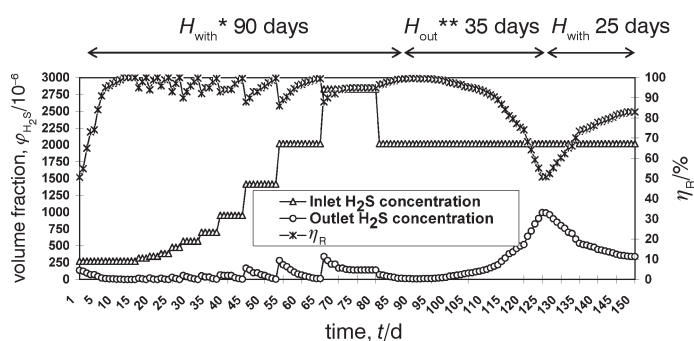
Fig. 5 – Change in removal efficiency with change in inlet H 2 S volume fraction during the entire 150 days of biofilter operation *With humidifier, **without humidifier
