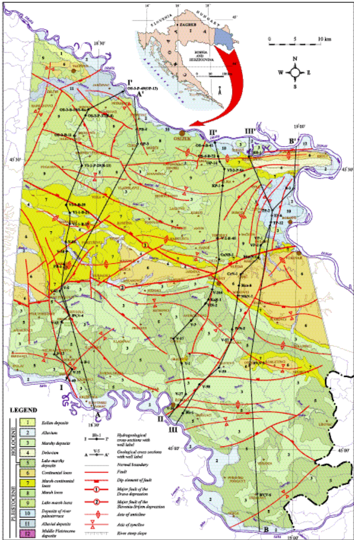
Fig. 1 Geological map.
