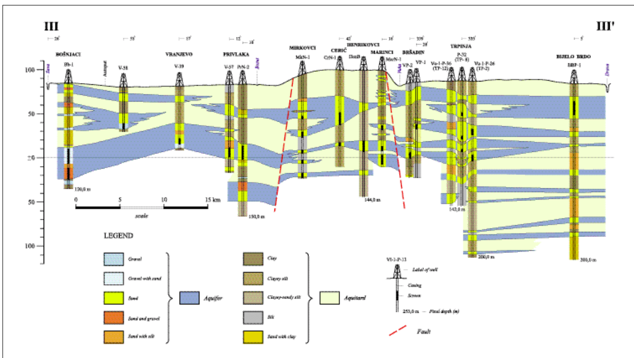
Fig. 5 Hydrogeological cross-section III-III'.
