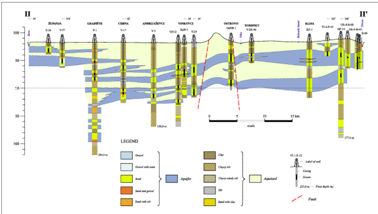
Fig. 4 Hydrogeological cross-section II-II'.
