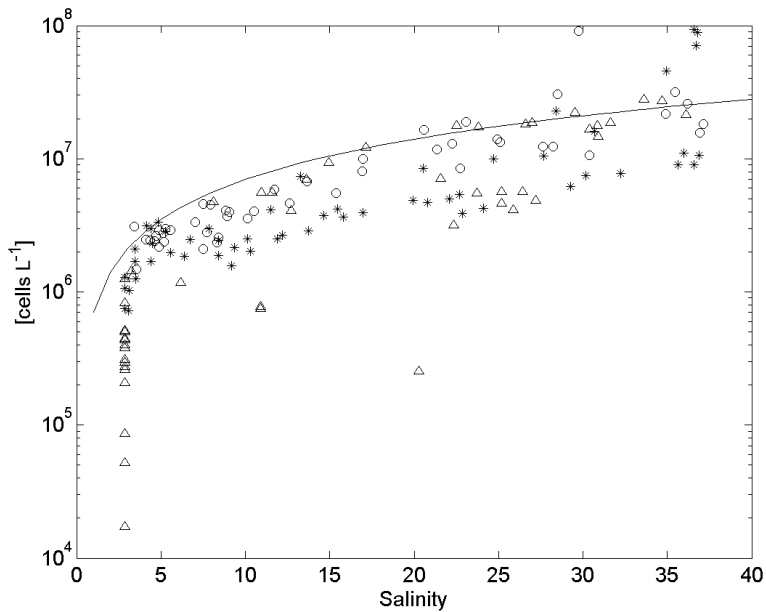
Fig. 4. The relationship between picocyanobacteria abundance and salinity in July (o), October (*) and February ( \Delta ) in the Ebro Estuary.
