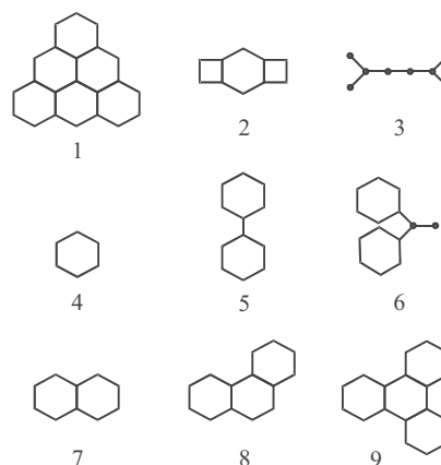
Figure 1. Examples of energy-poor (1-3) and energy-rich (4-9) conjugated hydrocarbons. The energy-poor systems 1 and 3 are non-Kekuléan. The Kekulé structure count of 2 is equal to four, but its algebraic structure count 1 is zero. Compounds 5 and 6 are characteristic representatives of energy-rich conjugated hydrocarbons. These have highly non-planar geometries and are therefore not suitable for the application of HMO theory (including the McClelland-number-concept). Compounds 7-9 seem to be the only stable planar polycyclic conjugated hydrocarbons with McClelland number different from 3.
