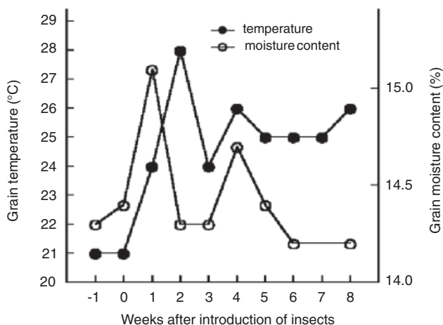
Figure 1 Weekly grain temperature and moisture content in the reference container
