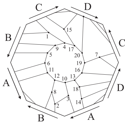
Figure 22. Sn9 embedded into double torus
