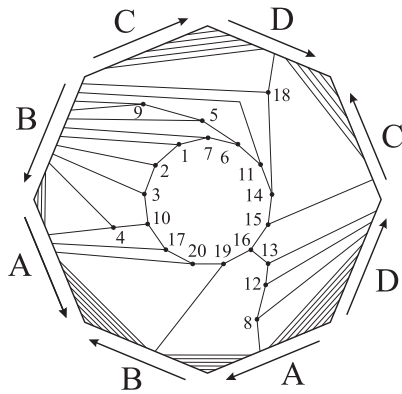
Figure 21. Sn8 embedded into double torus
