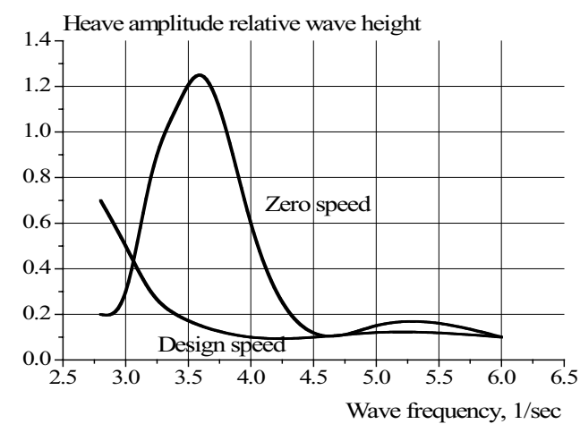
Figure 10 Response amplitude operator of heave in head waves Slika 10 Operator amplitude odziva kod poniranja na valovima u pramac
