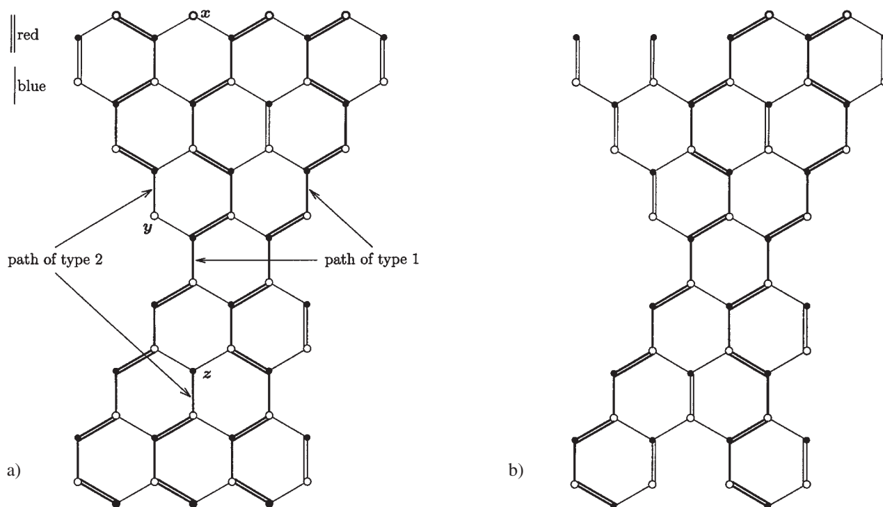
Figure 6. a) Hexagonal system H with one of its maximum matchings M (||). Vertices x , y , z not covered by M . n = 55 , m = 26 . b) Induced subgraph H^* of H with perfect matching M^* . n^* = 52 , m^* = m = 26 .
