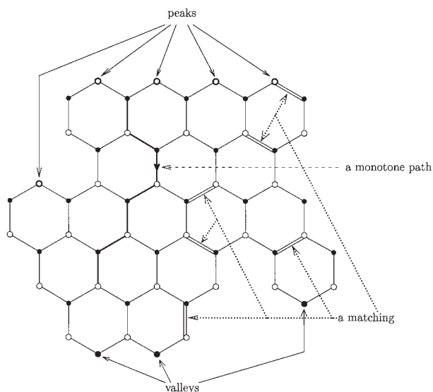
Figure 2. A hexagonal system.
