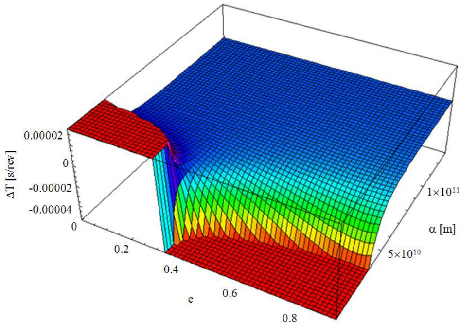
Fig. 5. The anomalous period time change of the planet HD 80606 b due to Lense-Thirring effect as a function of e and a by supposing that their values are altered in the ranges [0,1] and [\text{periastron-apoastron}] , respectively. An equatorial orbit case ( i = 0 ) is considered
