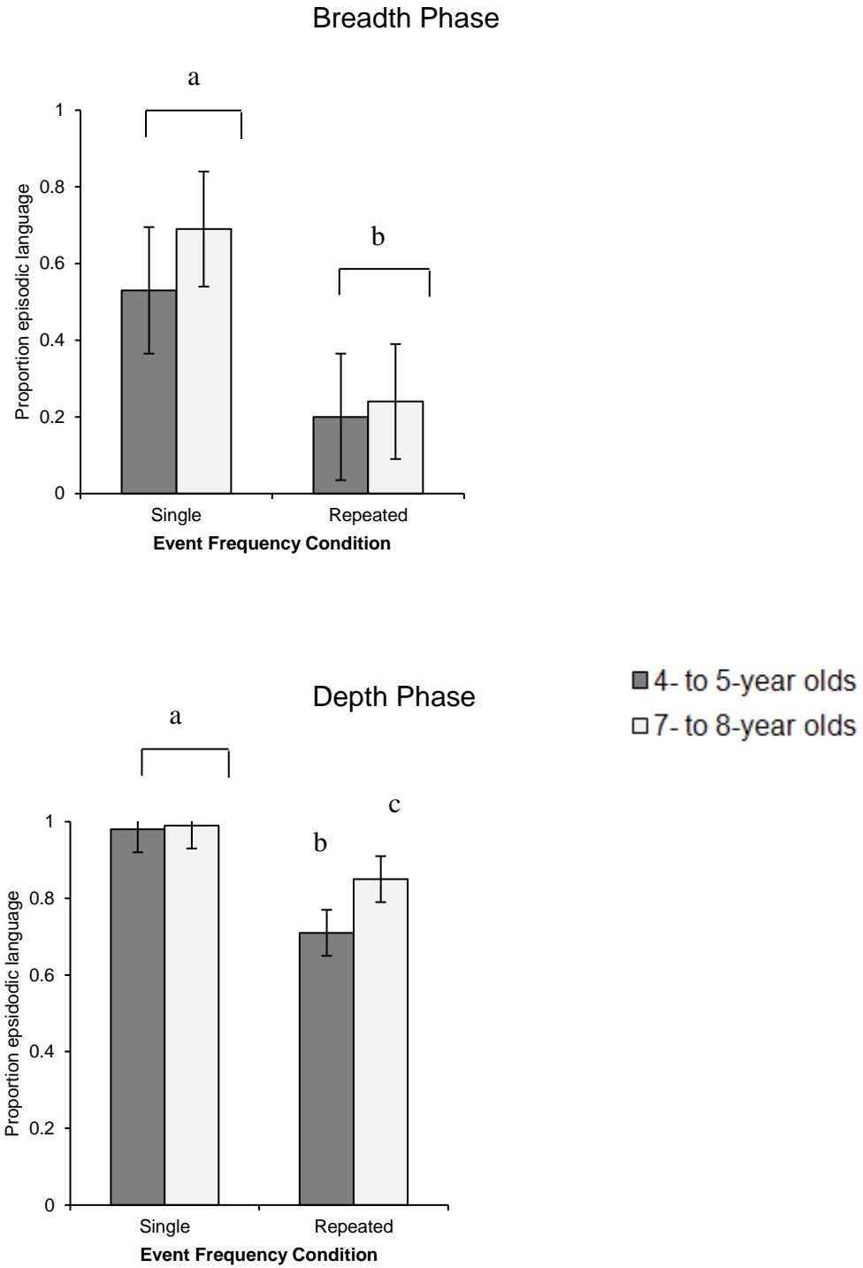
Figure 2. Three-way interaction among Age Group x Event Frequency x Phase on children`s language use.
